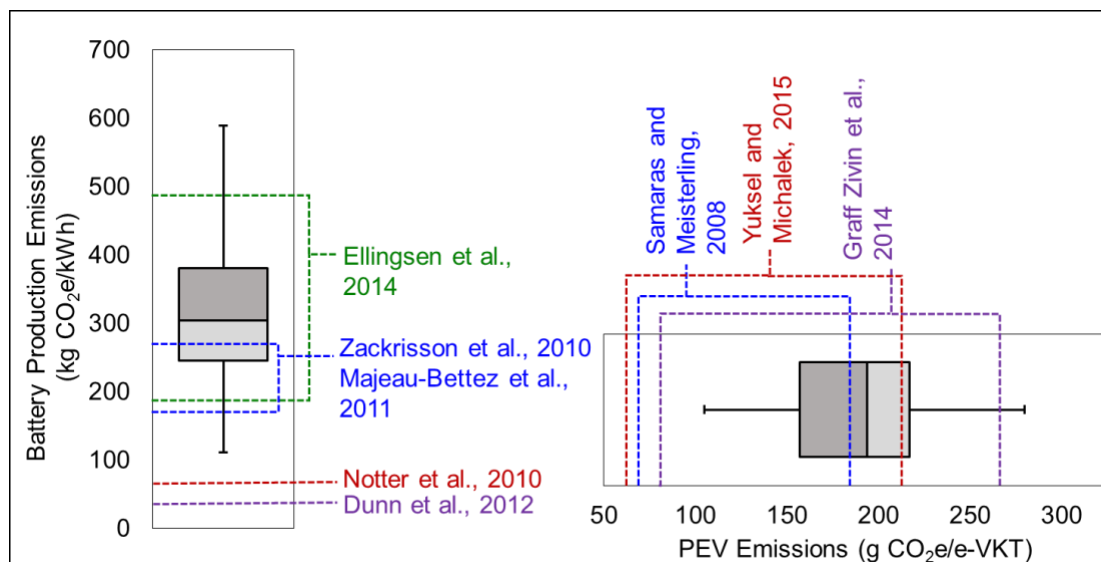
Figure 2. Comparing estimates for PEV and battery production emissions from previous studies [11, 12, 17-22], reproduced from [3]
