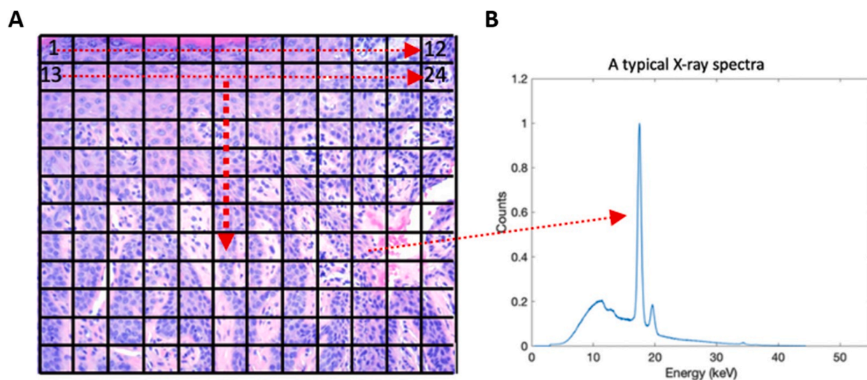
Fig. 3. (A) Pixel-by-pixel based scanning scheme with 60 s for each pixel (figure was donated by Dr. Chainani-Wu); (B) a schematic representation of a typical measured spectra from a typical pixel.
