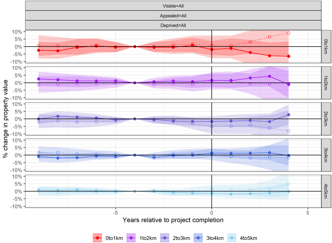
Figure 8: Commercial Capitalization Event Study for Solar Projects
