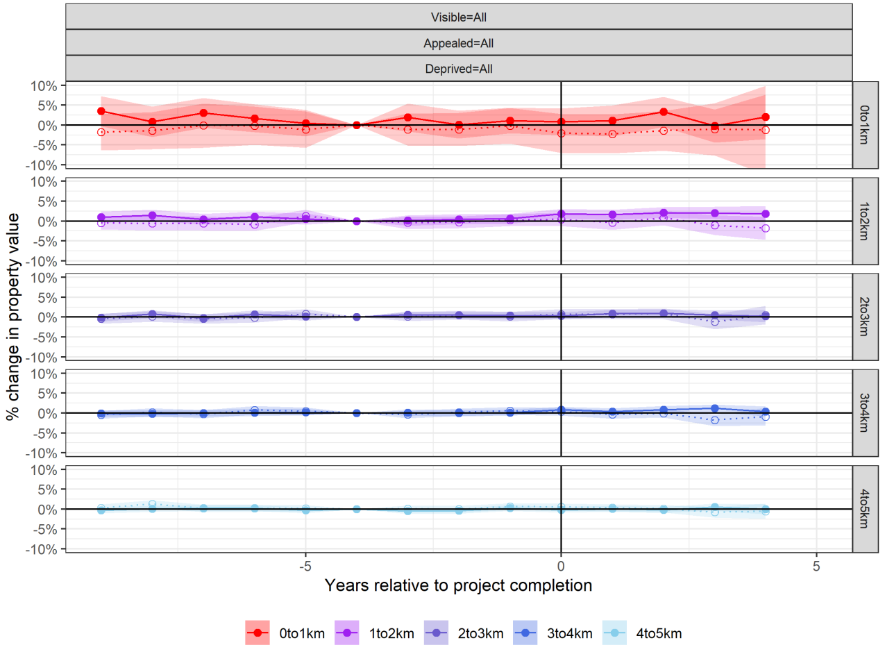
Figure 5: Residential Capitalization Event Study for Solar Projects
