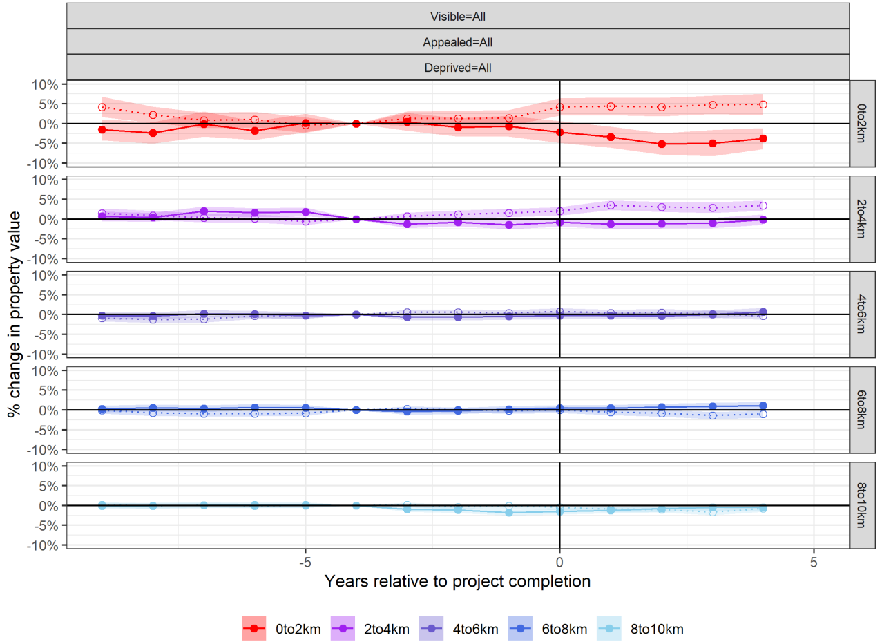
Figure 3: Residential Property Values Event Study Results for Wind Projects
