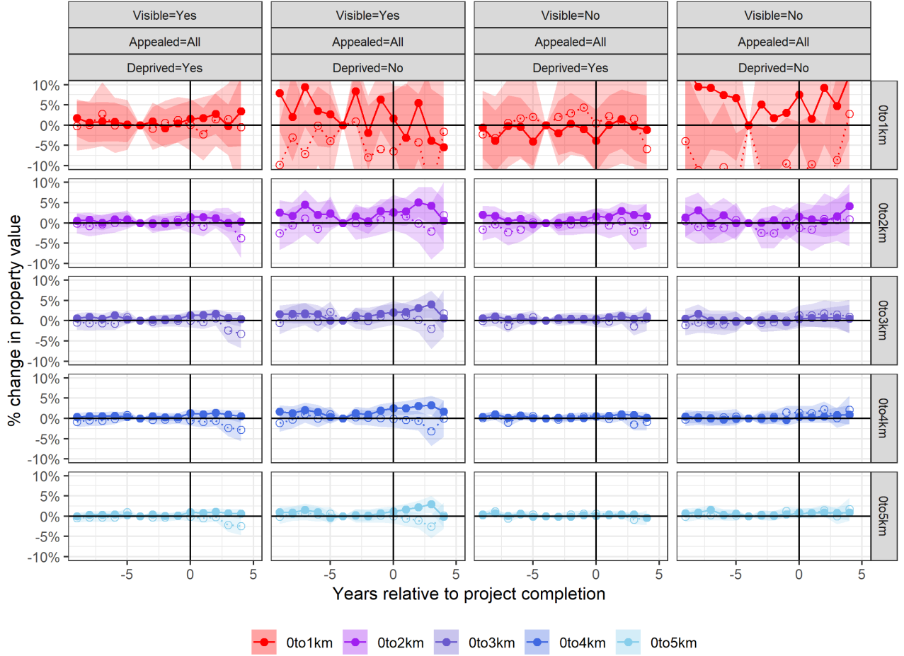
Figure 6: Residential Capitalization Event Study for Solar Projects with Differential Effects
