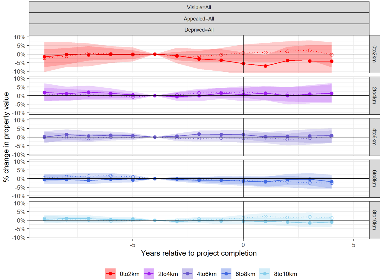
Figure 7: Commercial Capitalization Event Study for Wind Projects
