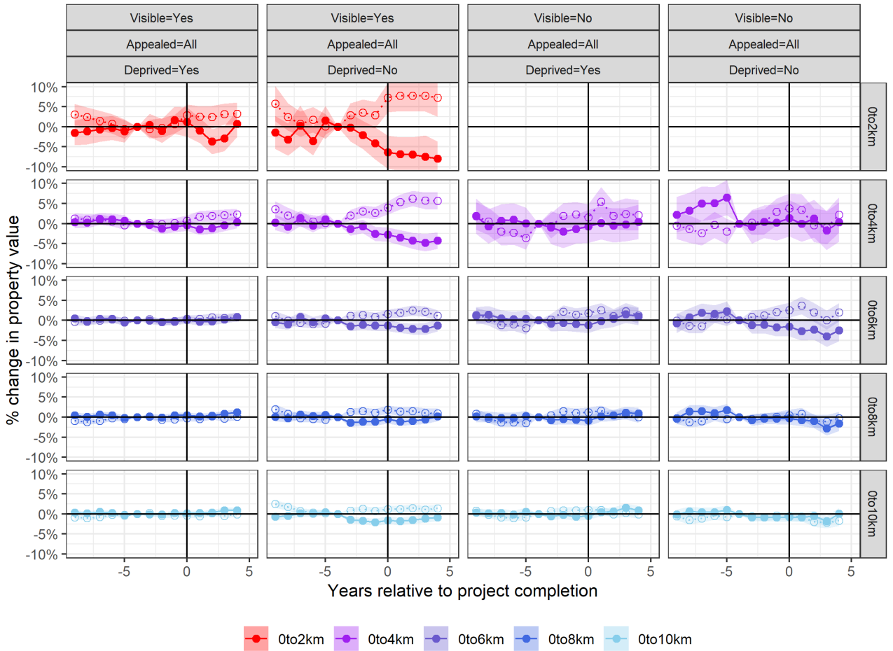
Figure 4: Residential Capitalization Event Study for Wind Projects with Differential Effects
