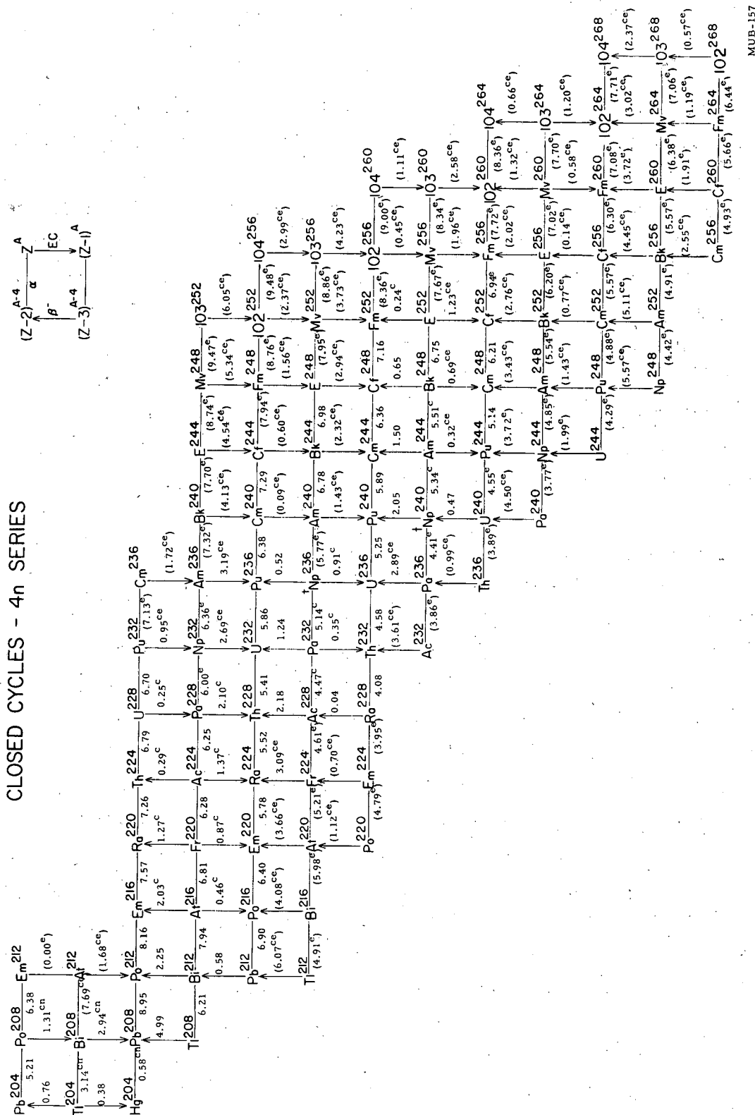
Fig. 2. Closed decay energy cycles for the 4n series: No superscript, measured energy; c, calculated; cn, calculated with neutron binding energies; e, estimated; ce, calculated from a cycle containing estimated energies; (-), uncertain by more than about 0.1 Mev; †, isomers.
