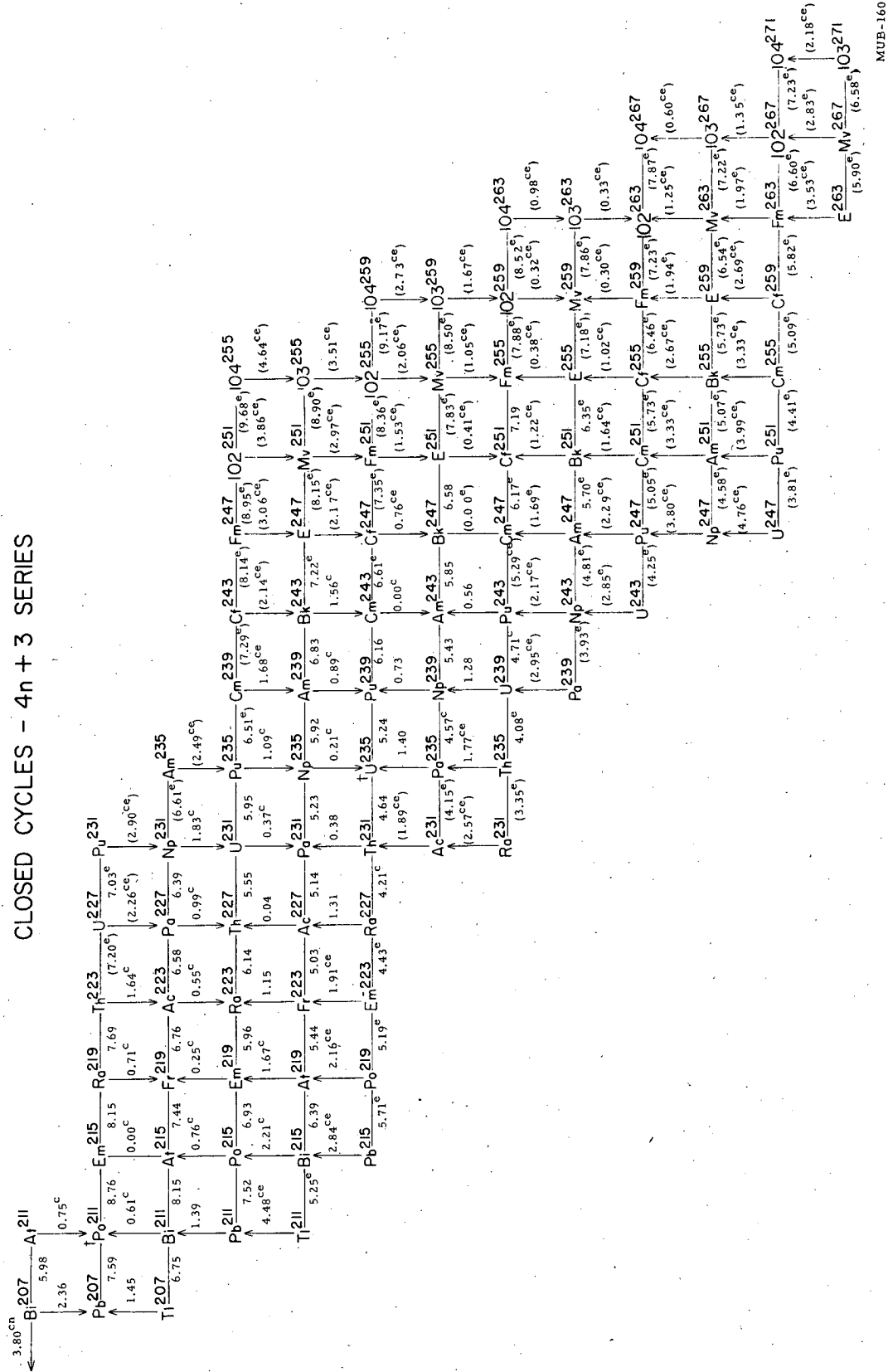
Fig. 5. Closed decay energy cycles for the 4n+3 series: No superscript, measured energy; c, calculated; cn, calculated with neutron binding energies, e, estimated; ce, calculated from a cycle containing estimated energies; ( ), uncertain by more than about 0.1 Mev; t, isomers.
