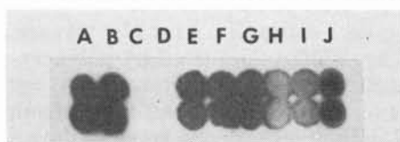
Fig. 5. Autoradiograph illustrating the results of the hybridization of 5' - ^{32} P-end-labelled citrus tristeza virus (CTV) double stranded (ds)RNA probe to purified nucleic acids or extracts from bark of sweet orange seedlings which have been spotted to nitrocellulose paper. Before spotting, CTV single stranded (ss) and dsRNAs were treated for 10 minutes at room temperature in 10mM methyl mercury hydroxide (MMH) in 50mM borate buffer. Bark was extracted in 1.5% sodium dodecyl sulphate in borate buffer. Extract supernatants were treated with MMH before spotting. All samples were run in duplicate: (A) CTV ssRNA; (B) CTV dsRNA; (C, D) extracts from uninoculated plants; and (E-J) extracts from one of 6 different isolates of CTV. Spotted paper was incubated in 5' -end labelled CTV dsRNA probe, and hybridization of probe to specific dots was detected by autoradiography. Details of methods have been published (7, 10).
