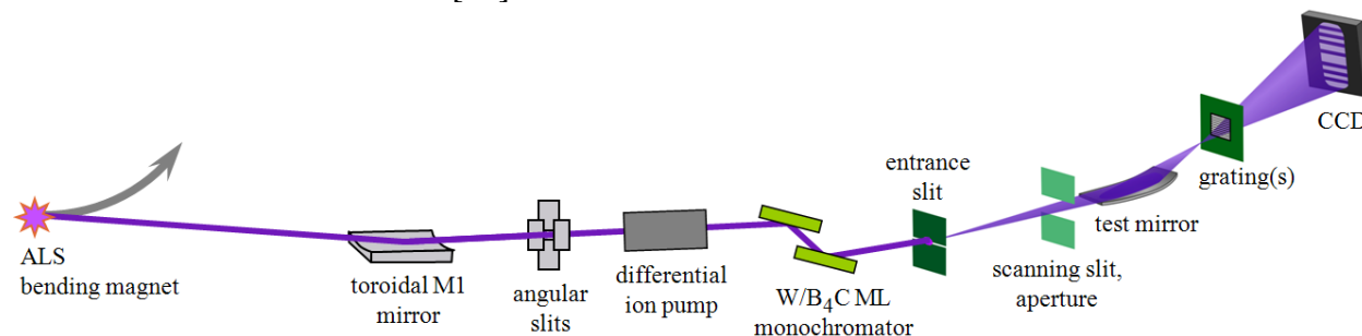
Figure 1: Beamline 5.3.1 arrangement
