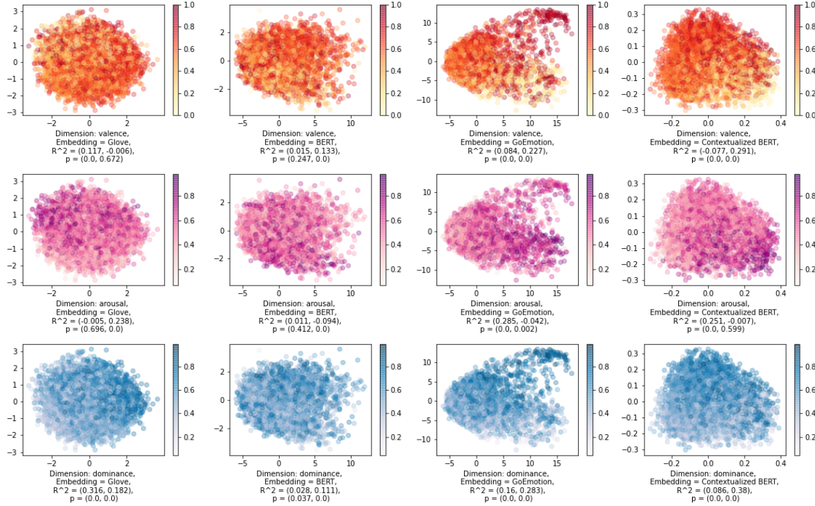
Figure 1: 2-components PCA representations of GloVe, base BERT, GoEmotion BERT, and contextualized BERT & human ratings for valence, arousal, and dominance (Human ratings were color-coded in a spectrum. Each dot represents a word. 5,586 words are represented. The darker the dot, the more prominent the human rating in the respective dimension.)
