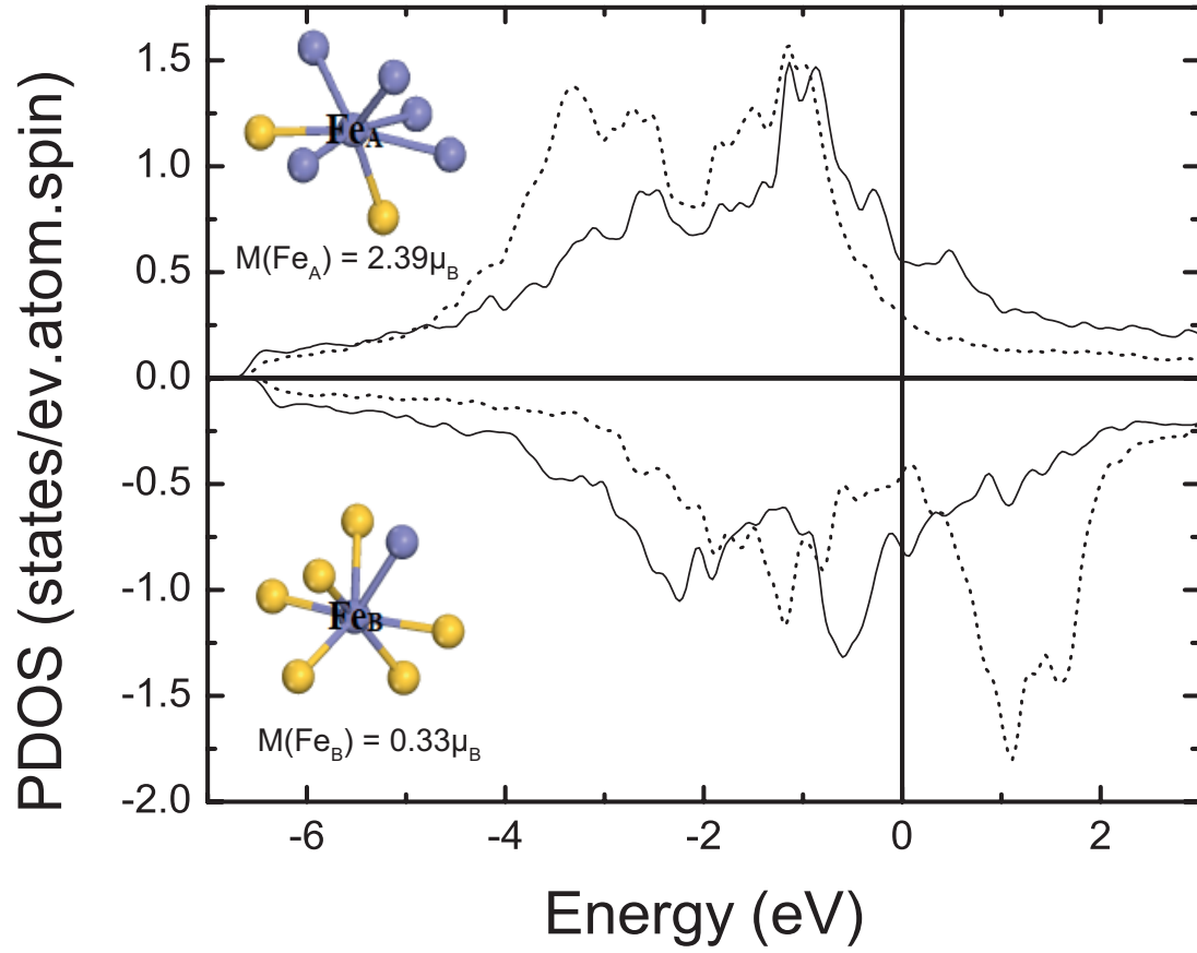
Figure S4. Partial density of states (PDOS) for two Fe atoms (Fe A and Fe B ) in the amorphous structure with different numbers of Fe and Si nearest neighbors, as shown. The Fe atoms are blue, and the Si atoms are yellow in the inset. The dashed (solid) PDOS corresponds to Fe A (Fe B ).
