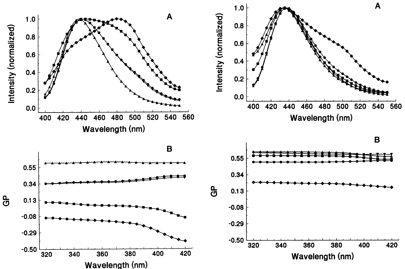
FIGURE 2 Normalized laurdan fluorescence emission spectra (A) and excitation GP spectra (B) in multilamellar phospholipid vesicles composed of 30 mol% cholesterol and DOPC ( \blacklozenge ), DLPC ( \bullet ), DPPC ( \blacktriangledown ) and of equimolar mixtures of DOPC and DPPC ( \blacktriangledown ) and of DLPC and DPPC ( \blacksquare ) at 20°C.
