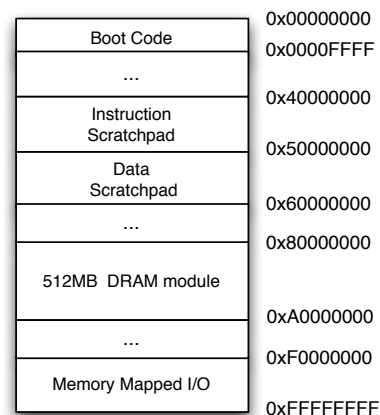
Figure 3.3: Memory Layout of PTARM
