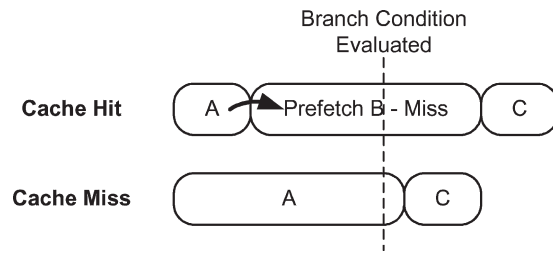
Figure 1.3: Timing anomaly cause by speculation [97]
