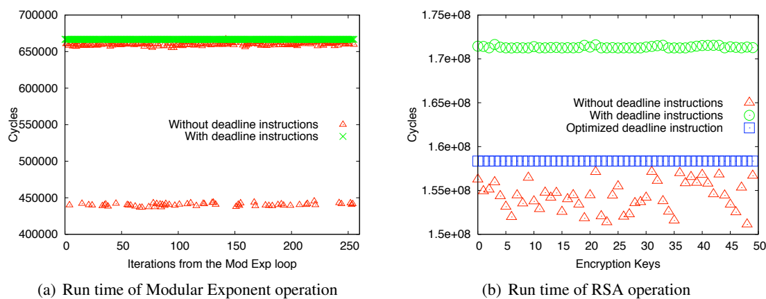
Figure 4.8: RSA Algorithm
