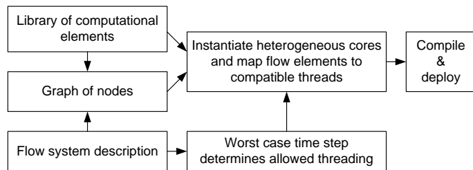
Figure 4.1: Design Flow
