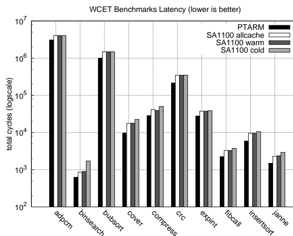
Figure 3.17: Malardalen benchmarks latency
