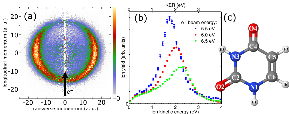
Figure 2: (a) Measured ion momentum distribution, in atomic units (a. u.), of \text{H}^- resulting from DEA to uracil at an electron beam energy of 6.0 eV. The electron beam direction is indicated by an arrow. Inset: the equilibrium geometry of uracil with site labels adopted in the text. (b) Kinetic energy distribution of \text{H}^- ions for the electron beam energies indicated, normalized for each electron incident energy to the cross section data of Ref. 13. Error bars indicate one standard deviation of the statistical uncertainty and the intensity scales are linear with arbitrary units.
