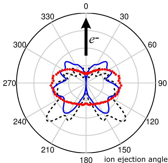
Figure 3: Polar plot of the measured (red circles) \text{H}^- anion fragment ion yield (radial coordinate) as a function of the ejection angle (angular coordinate); orientationally averaged square modulus of the entrance amplitude as a function of the angle \theta between the electrons direction of incidence and the direction of the N1-H1 bond (continuous blue curve) and the N3-H3 bond (dashed black curve), with \theta = 0^\circ corresponding to the incident electron direction \vec{k}_{in} .
