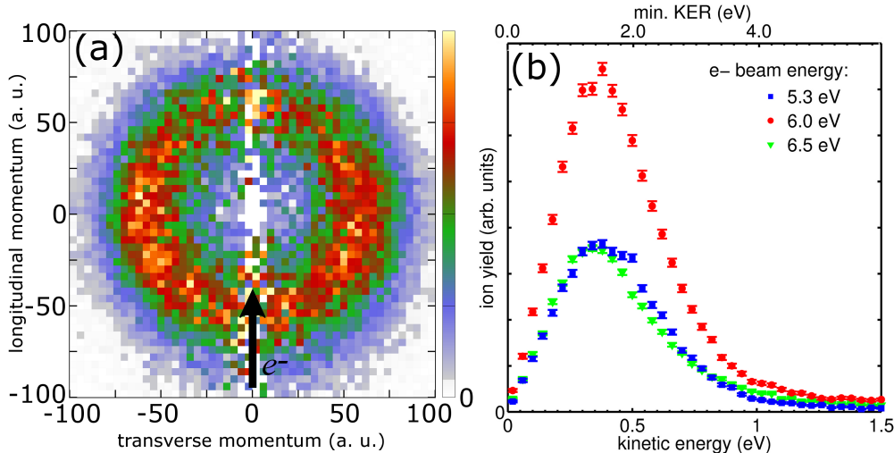
Figure 4: (a) As Fig. 2, for \text{C}_3\text{H}_3\text{N}_2\text{O}^- at an electron beam energy of 6.0 eV. (b) As Fig. 2, kinetic energy and minimum KER distribution of \text{C}_3\text{H}_3\text{N}_2\text{O}^- following DEA to uracil at the specified energies near 6.0 eV.
