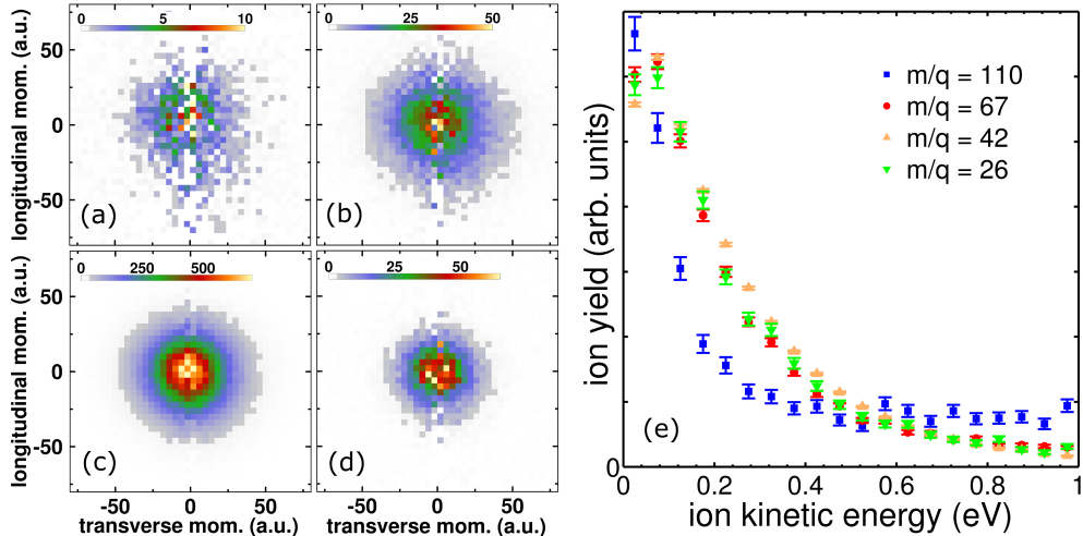
Figure 1: Measured ion momentum distribution following DEA to uracil at 6.0 eV electron energy (a) 110 atomic mass units (amu), C_4H_2N_2O_2^- , (b) 67 amu, C_3HNO^- , (c) 42 amu, NCO^- , and (d) 26 amu, CN^- . The electron beam direction is longitudinal from bottom to top and the linear color scales represent ion counts in arbitrary units. (e) Ion kinetic energy for each channel in (a) - (d). Error bars represent one standard deviation of the statistical uncertainty.
