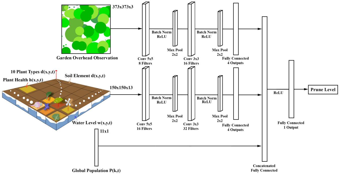
Fig. 5. Learned Pruning network architecture. A deep convolutional neural network with 18,244 parameters. The network takes three inputs: 1) an RGB image of the full garden; 2) a matrix of h(x, y, t) , w(x, y, t) and \mathbf{d}(x, y, t) for all (x, y) in the garden; 3) the global population distribution \mathbf{P}(k, t) including soil coverage. The network predicts a prune level for each observation using demonstrations from Variable Pruning.
