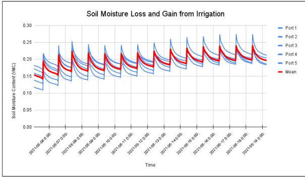
Fig. 4. Soil moisture curve generated from TEROS-10 soil moisture sensors connected to a data logger to determine water loss and gain rates. Irrigation was applied every 24 hours. Soil moisture readings were recorded every 30 minutes. The five blue curves represent five different sensors that were each watered independently. The red curve is the average of the readings of all five sensors.
