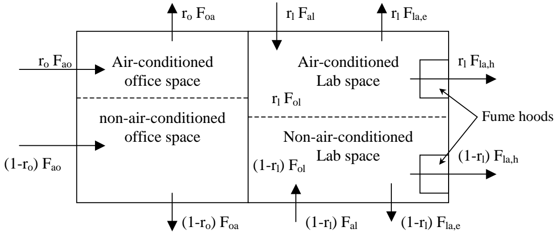
Figure 1: Schematic diagram of the laboratory building.
