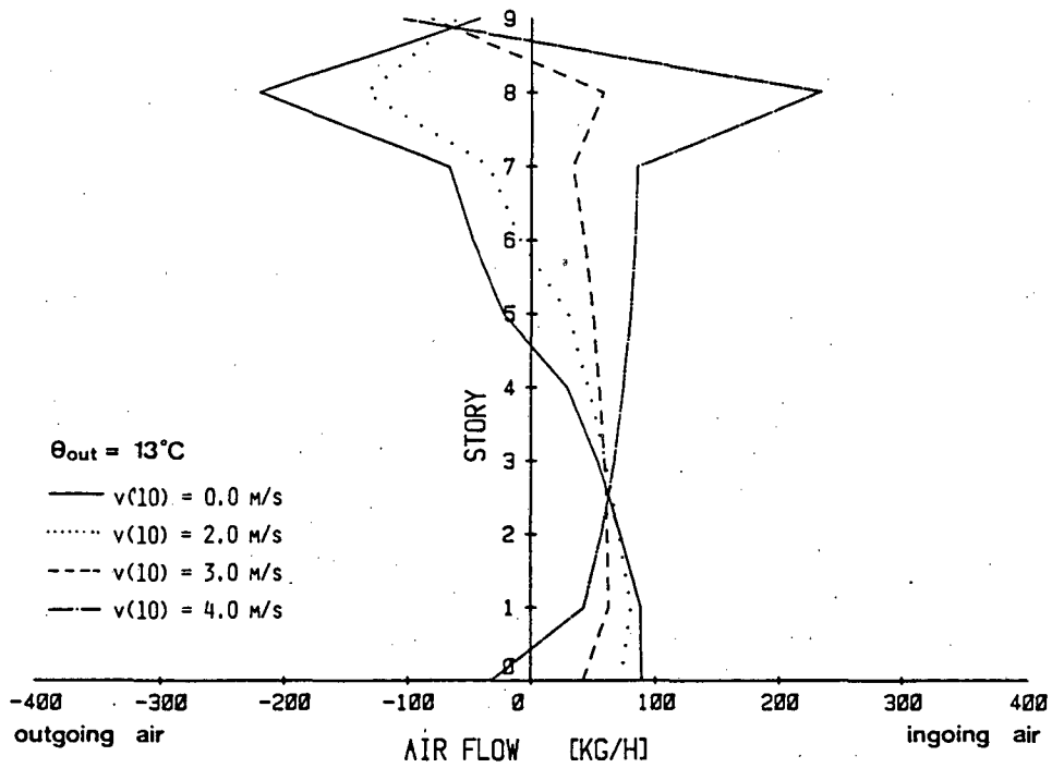
Fig. 6(a). Computer calculated in-/exfiltration flows from the staircase through air leakages in the outside surface of the building as a function of the building height ( \Theta_{out} = 13^\circ\text{C} ).
