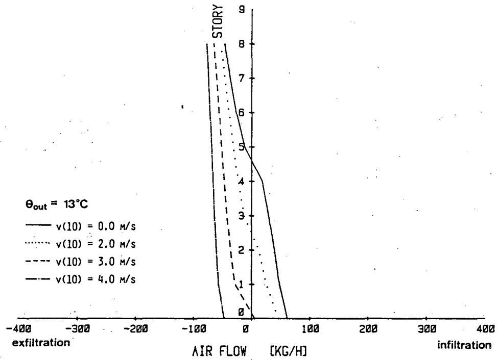
Fig. 7. Wind effect onto the air current from the corridors to the staircase at different floor levels ( \theta_{out} = 13^{\circ}\text{C} ).
