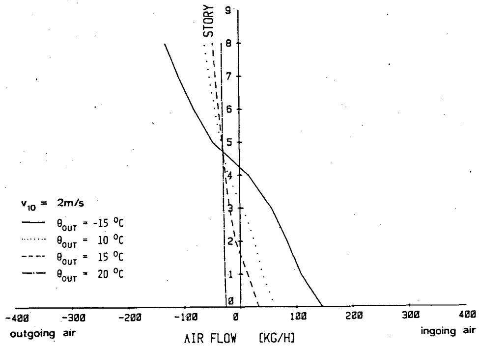
Fig. 8. Influence of ambient air temperature changes onto the air flow to the staircase from different floors ( v_{wind} = 2 \text{ m/s} ).
