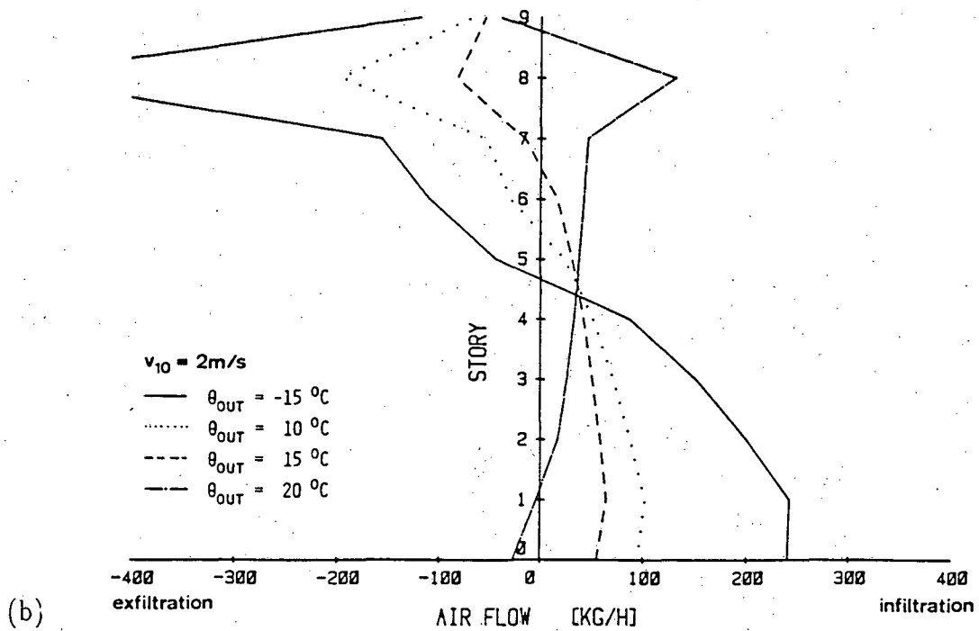
Fig. 9. Temperature and height dependence of: (a) total air flow into the building; (b) air current through elevator shaft doors (windspeed: v(10) = 2\text{ m/s} ).
