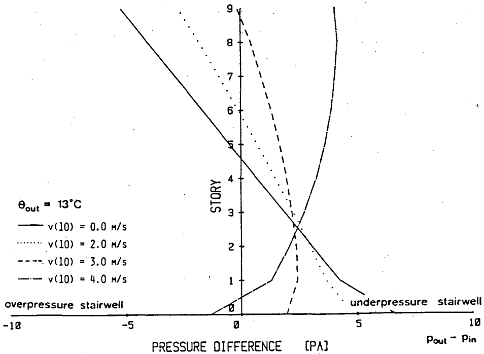
Fig. 6(b). Computer calculated driving pressure forces \Delta p = p_{out} - p_{in} as function of the building height ( \Theta_{out} = 13^\circ\text{C} ).
