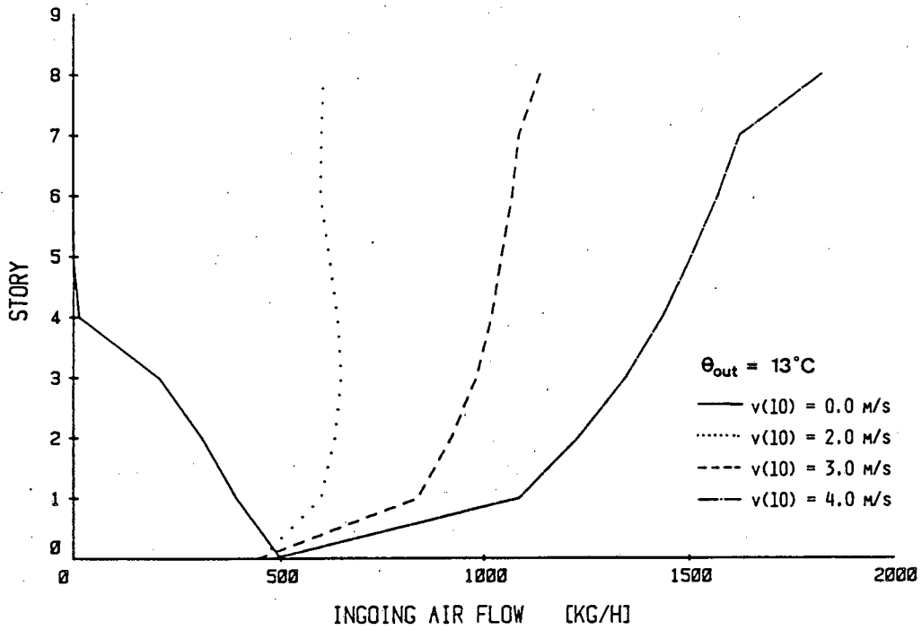
Fig. 4. Influence of the wind velocity on the air flowing into the building ( \theta_{out} = 13^{\circ}C ).
