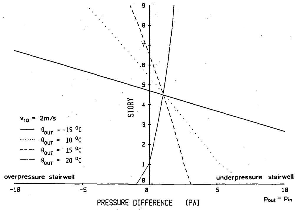
Fig. 9. Temperature and height dependence of: (c) air flow through openings in the outside surface of the staircase; (d) pressure differences between windward building facade and staircase (wind speed: v(10) = 2\text{ m/s} ).
