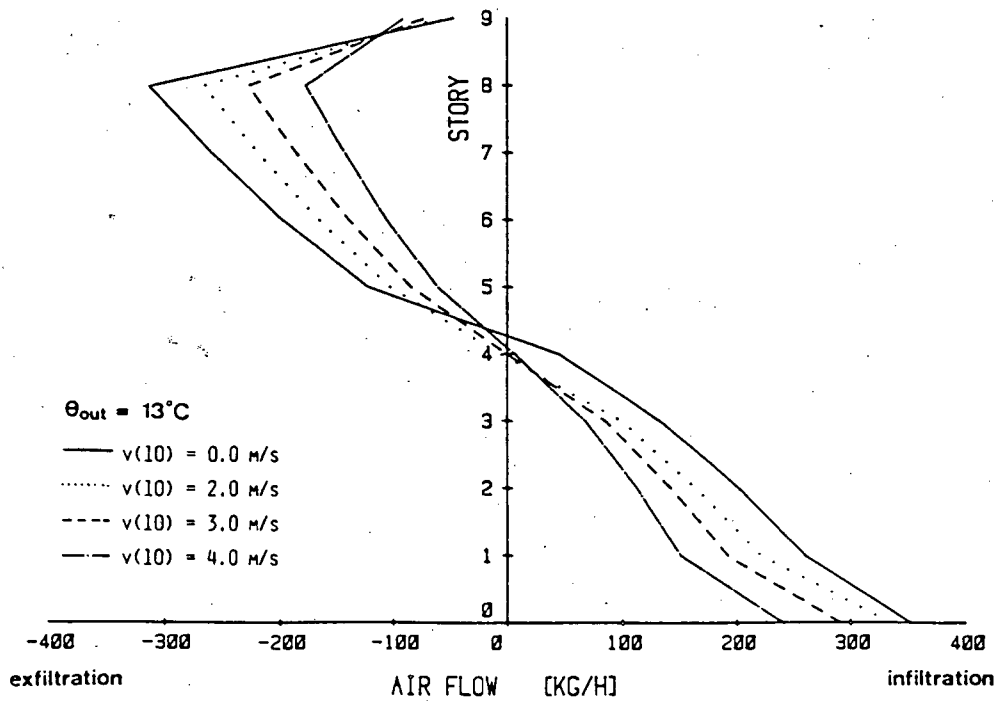
Fig. 5. Air flow through openings of the elevator shaft for different wind speeds ( \theta_{out} = 13^{\circ}C ).
