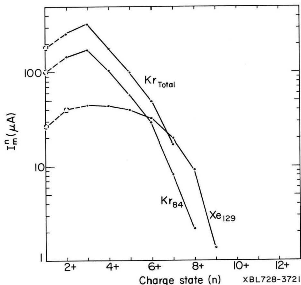
2.9 amp arc at 24%. U = 16KV, 100KV/cm. 4x40mm. collimation. Gas flow unrecorded. Kr +1 , Xe +1 , Xe +2 estimated.
