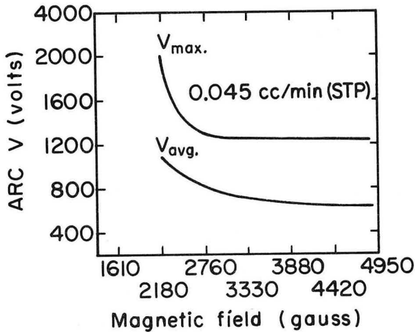
3 amp Krypton arc (24%). Magnetic field measured on centerline of source axis. V_{max} = peak arc potential at beginning of pulse. V_{avg} = average arc potential.
