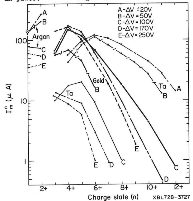
3 amp arc at 24%. U = 12KV, 120KV/cm. 0.03cc/min argon, (STP). 13x50mm collimation.
