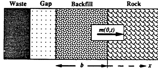
Figure 1b. Release of Soluble Species into Backfill and Rock
