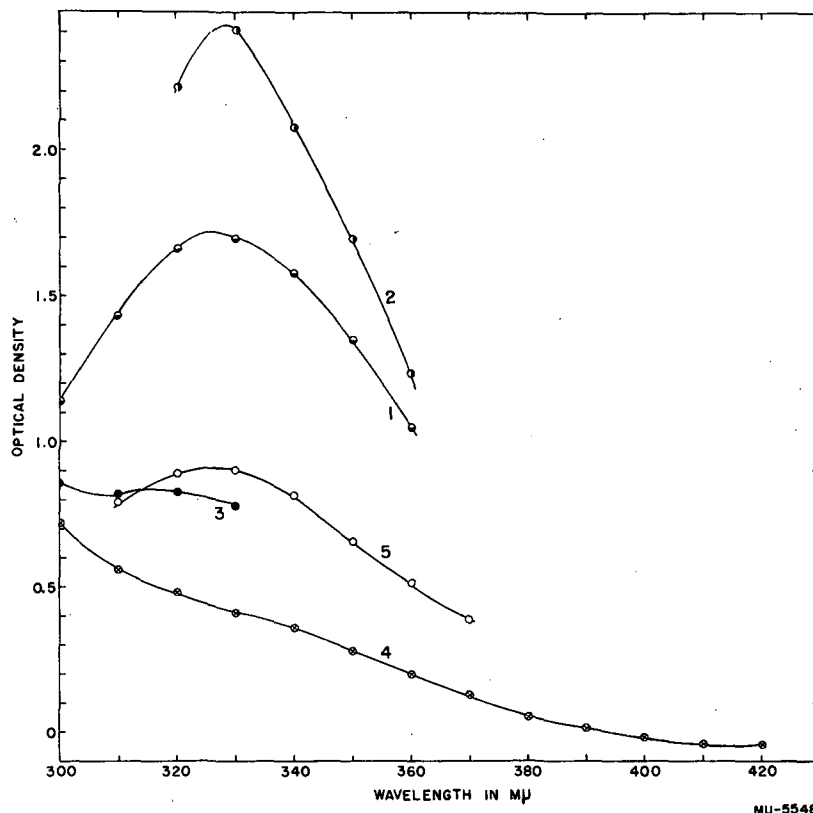
LOW TEMPERATURE PHOTOLYSIS OF TRIMETHYLENE DISULFIDE
