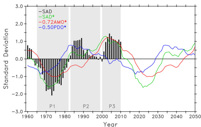
Figure 5. Projections of SAD (SAD*; green), AMO (AMO*; red), and PDO (PDO*; blue) to the year 2050, with the original SAD (black).
