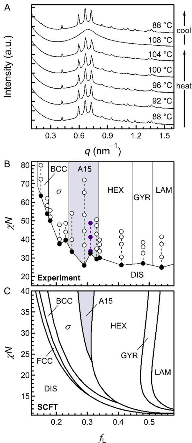
Fig. 3. Phase behavior of DL diblock copolymers. (A) A15 forms reversibly in DL-76 as evidenced by dynamic heating (1 °C/min) and cooling through the T_{\text{ODT}} \sim 105 °C. (B) The experimental DL phase diagram reveals a region of A15 stability approximately f_L = 0.25 – 0.33 ; phase coexistence ( \sigma /A15 and A15/HEX) occurs near either f_L boundary. Points examined by SAXS are marked with open circles and (\chi N)_{\text{ODT}} identified with dynamic mechanical thermal analysis is indicated by filled black circles. Sample DL-76 from A is denoted with filled purple circles. (C) SCFT mean-field phase diagram mapped onto \chi N vs. f_L at \epsilon = 3 semiquantitatively matches experiments: \sigma , A15, and HEX phases occur over similar volume fraction ranges at large \chi N . The disagreement for \chi N < 30 arises due to composition fluctuations as addressed in Fig. 4 (see text for discussion).
