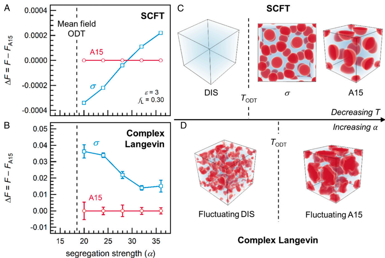
Fig. 4. Relative stability of the A15 and \sigma -phases (free energy in k_B T per chain differences) as calculated with (A) SCFT and (B) fully fluctuating complex Langevin field-theoretic simulations for f_L = 0.3 and invariant degree of polymerization N = 5,400 . Segregation strength in the model used for both SCFT and FTS is controlled by the parameter \alpha , which is related to \chi N . (C and D) Unit-cell renderings from (C) SCFT and (D) FTS highlight the different predicted temperature-dependent phase sequences, an effect of fluctuations; discrete, red domains are PLA-rich. Note that the BCC phase has been omitted from C for clarity.
