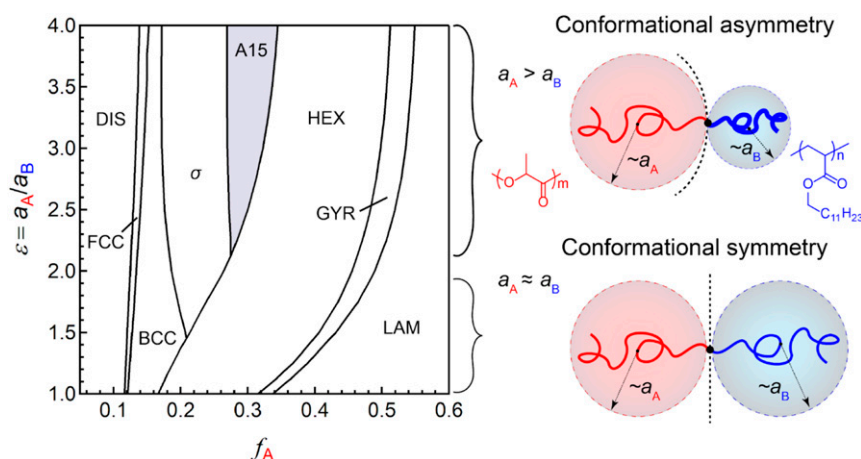
Fig. 1. ( Left ) SCFT simulations ( \chi N = 40 ) predict the A15 phase will be favored in AB diblock copolymers with sizable conformational asymmetry, \varepsilon \geq 2.1 . ( Right ) Illustration of the difference in pervaded block volumes that leads to large \varepsilon ; poly(dodecyl acrylate)– block –poly(lactide) accentuates this effect.
