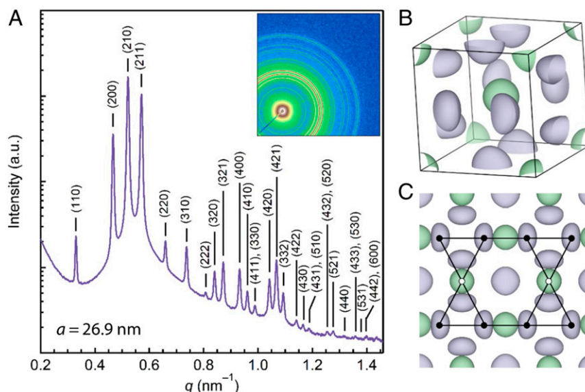
Fig. 2. Discovery of the A15 phase in DL diblock copolymers. (A) SAXS profile of A15 obtained with DL-120 (annealed at 125 °C for 19 h); all allowed reflections for space group Pm\bar{3}n out to (600) are demarcated with vertical lines ( a = 26.9 nm). (B) Unit-cell electron density reconstruction (78% isosurface) corresponding to the data in A; see SI Appendix for details. Two symmetry-distinct micelles (shape, volume) occupy Wyckoff positions 2a and 6d (false colored green and purple, respectively). (C) Projection of the electron density map along one a axis with an outline of the characteristic A15 tiling pattern containing two types of nodes— 3^2.6^2 (black circles) and 3.6.3.6 (white circles).
