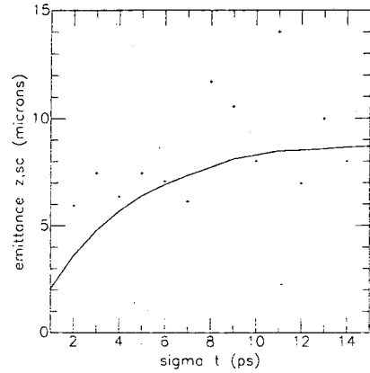
Fig. 6. The space-charge induced longitudinal emittance calculated from simulation (marked by +) and from theory (solid line).
