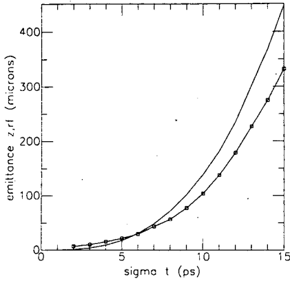
Fig. 4. The rf induced longitudinal emittance as a function of \sigma_t calculated from simulation (marked by \square ) and from theory (solid line).
