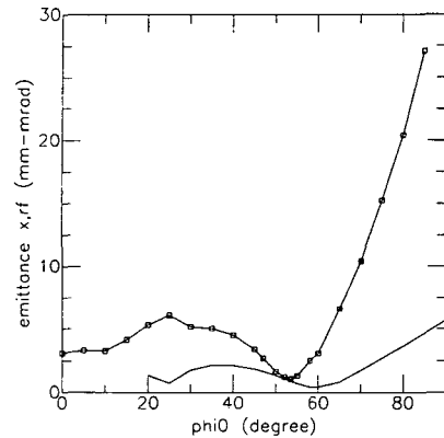
Fig. 3. The rf induced transverse emittance as a function of \phi_0 calculated from simulation (marked by \square ) and from theory (solid line).
