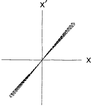
Fig. 2. Electron distribution in transverse phase space due to time-dependent focusing of the rf field.
