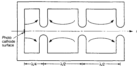
Fig. 1. Schematics of the rf laser gun.
