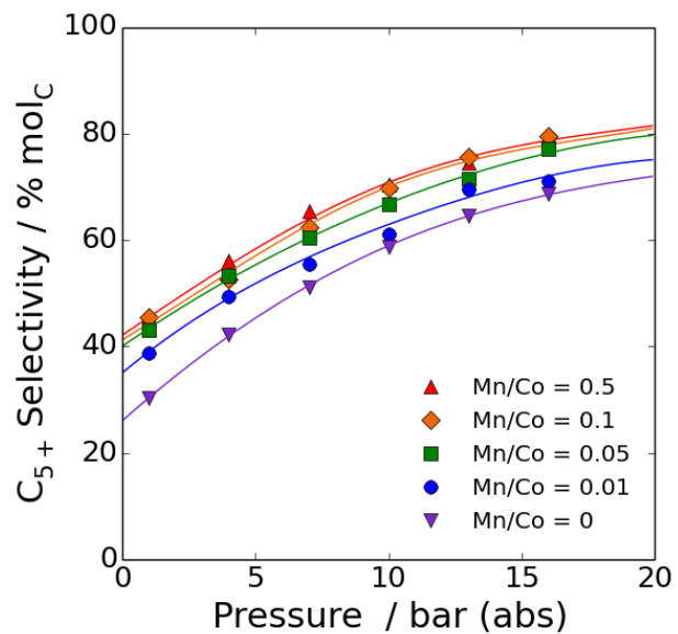
Figure 11. Comparison of (A) methane and (B) C 5+ selectivities as a function of pressure at 493 K for catalysts with different Mn/Co ratios. The data were extrapolated to 0 % conversion. The curves in the plots are cubic splines intended for visual aid.
