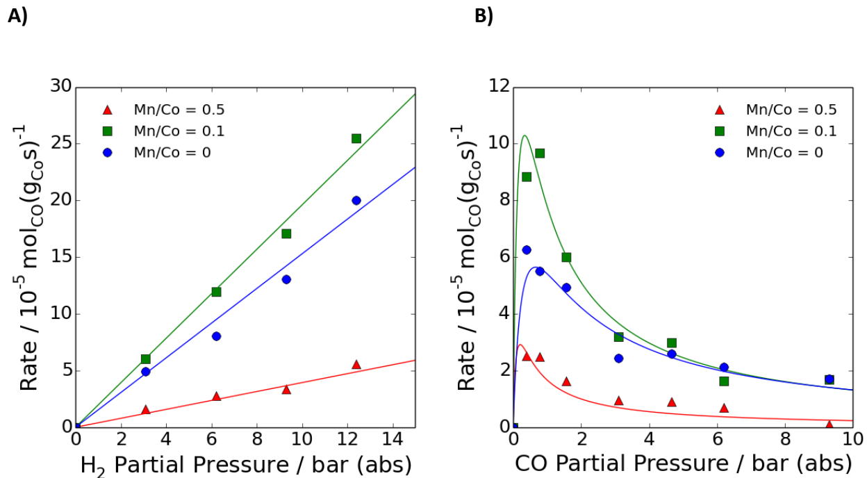
Figure 8. Dependence of CO consumption rate on (A) H 2 and (B) CO partial pressures. The variation of H 2 partial pressure was done with a constant CO partial pressure of 1.55 bar; the variation of CO partial pressure was done with a constant H 2 partial pressure of 3.1 bar. The data for both figures were collected at 493 K and were extrapolated to 0 % conversion. The curves in the plots correspond to the rate law from Eq. (3) fitted to the data.
