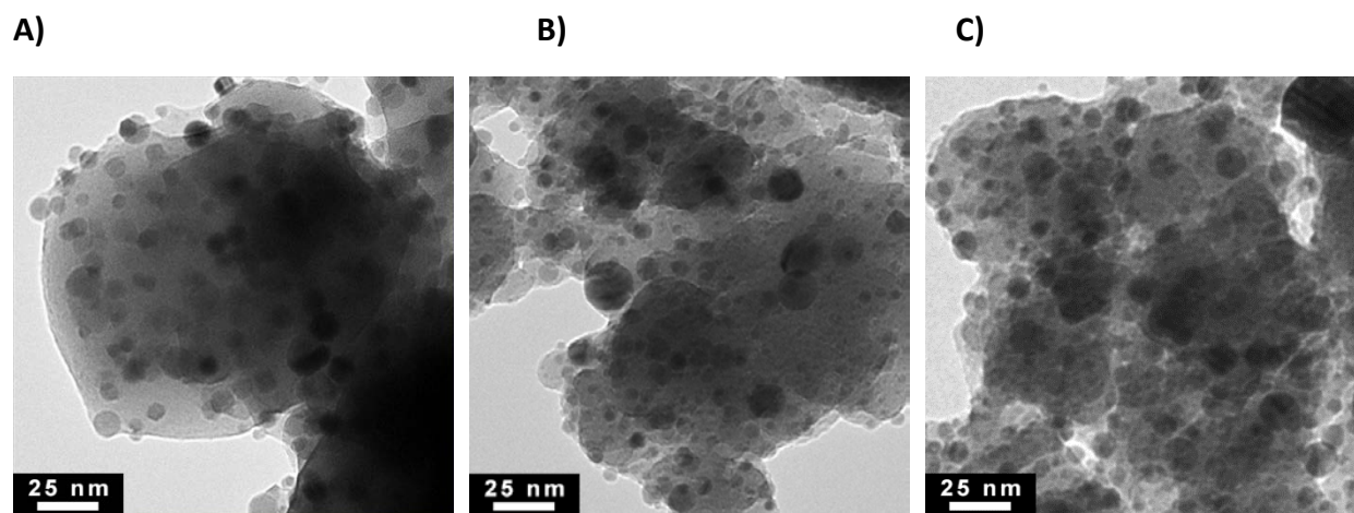
Figure 1. Bright-field TEM images of Co-Mn catalysts with bulk Mn/Co atomic ratios of (A) Mn/Co = 0, (B) Mn/Co = 0.1, and (C) Mn/Co = 0.5. For all catalysts, the Co loadings were 10 wt% relative to Co and silica. Particle size distribution statistics are reported in Table 1.
