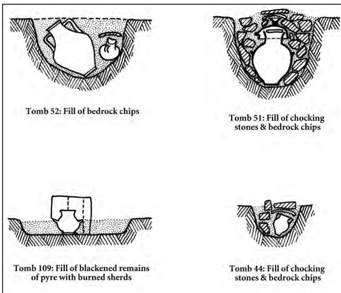
FIGURE 14 (on facing page). Sketch sections of some typical cremation tombs (not to scale).
