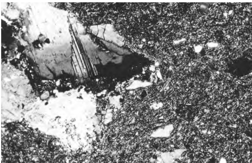
PLATE 538. Microstructure of clay sample C4, from lagoon to the north of Torone; fired at 700°C. Width of photograph is 3.2mm.
