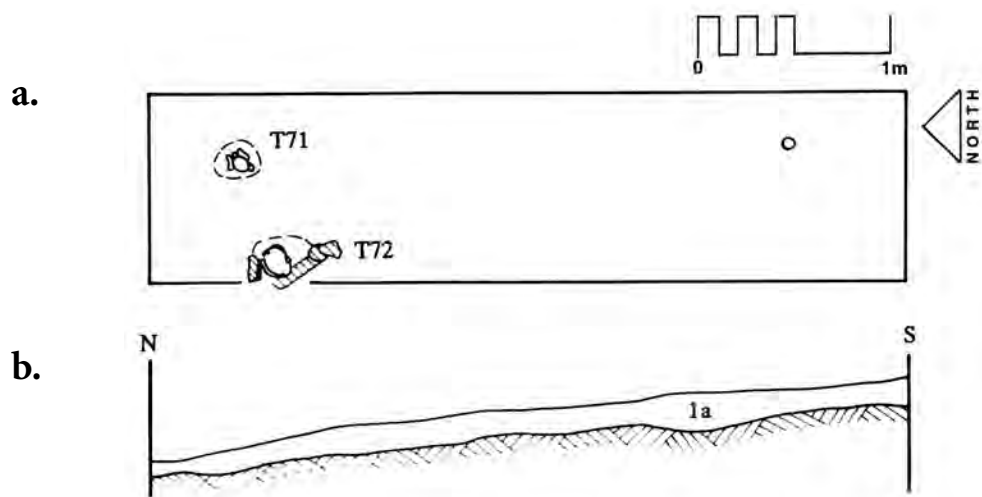
FIGURE 41. Trench 46 East Baulk. (a) Plan. (b) Section.
