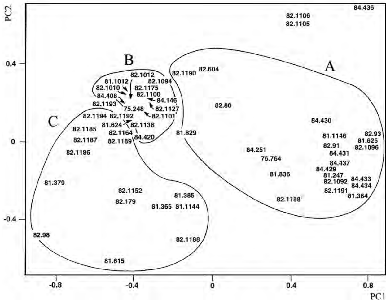
FIGURE 223. Principal components plot (PC1 vs. PC2) of the chemical data (all elements except Si and Ti) for all samples excluding T99-1 . The three clusters (A, B, and C) observed in fig. 224 have been superimposed. In the dendrogram KP-13 belongs to cluster C. The boundary of cluster A is drawn to indicate that the cluster includes three outliers ( 53 , 54 and T101-8 ).
