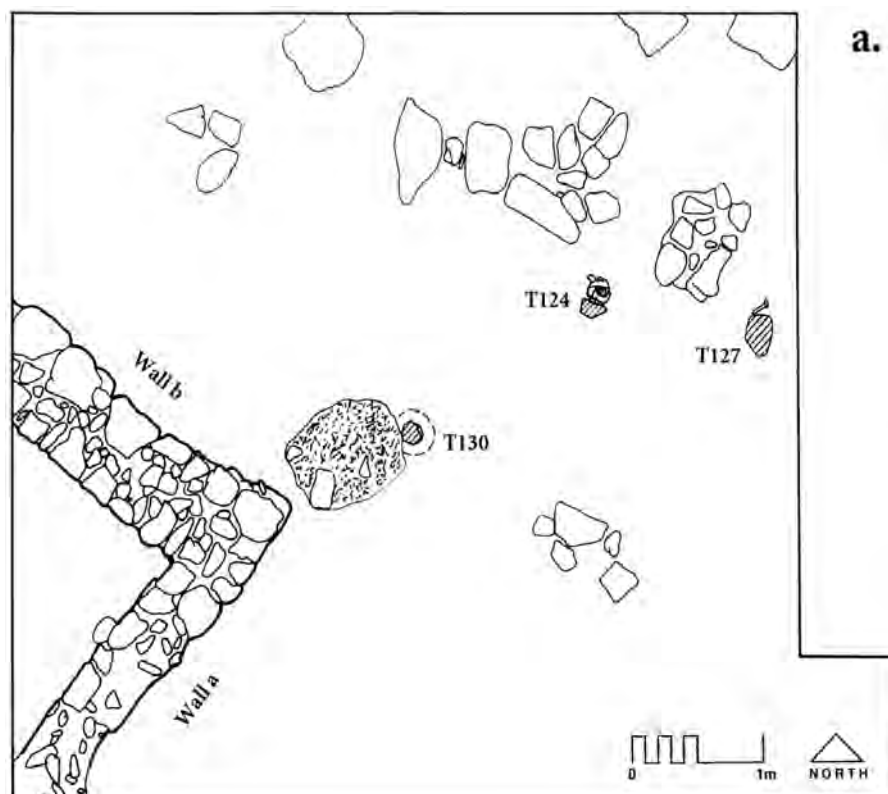
FIGURE 23 (on facing page). Trench 9. (a) Plan (Stage 1) showing covered tombs and Classical walls, paving stones, and tumble. (b) Plan (Stage 2) showing Early Iron Age tombs uncovered.
