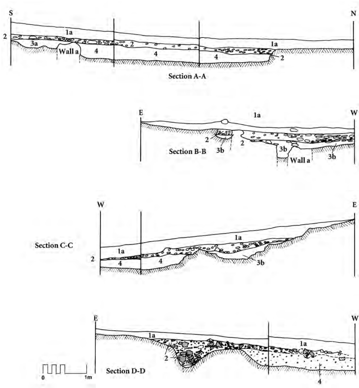
FIGURE 24 (continued). Trench 12. (b) Sections.
