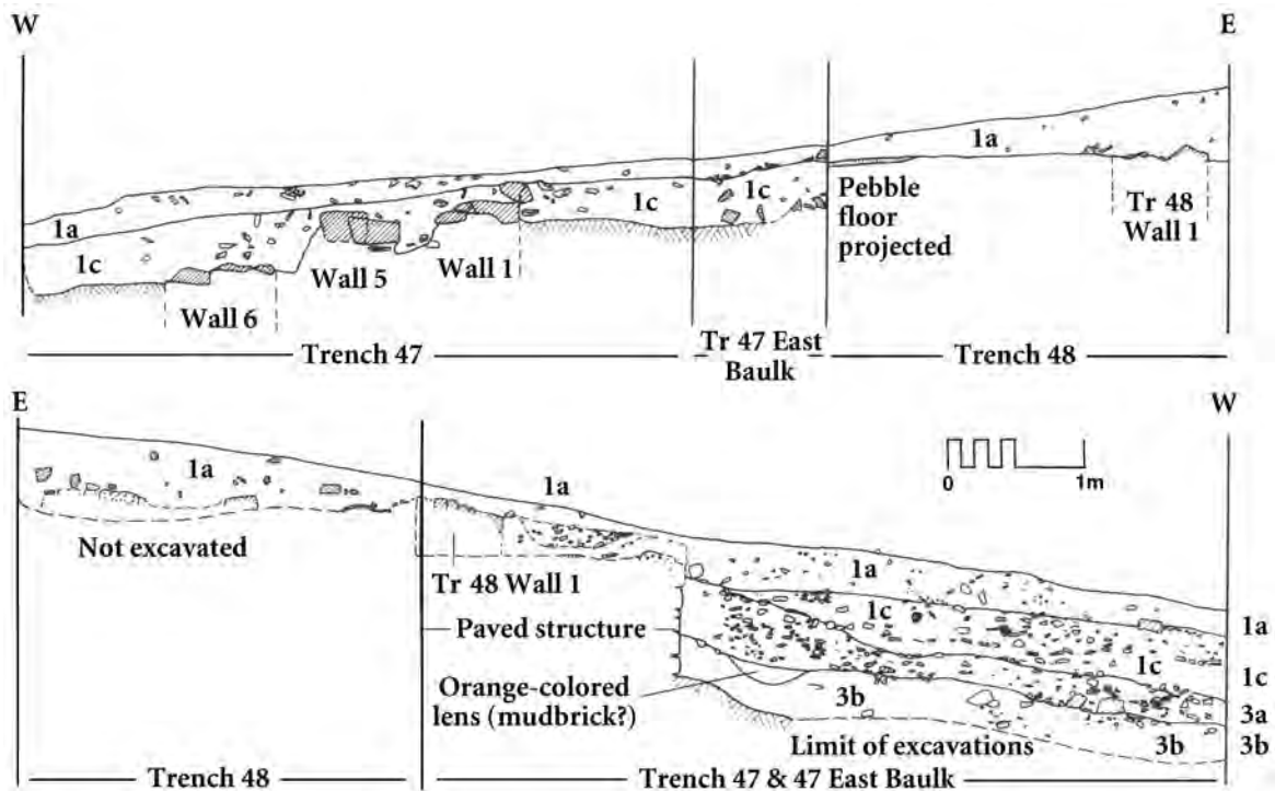
FIGURE 45. Trenches 47, 47 East Baulk, and 48. Sections (north and south scarps).
