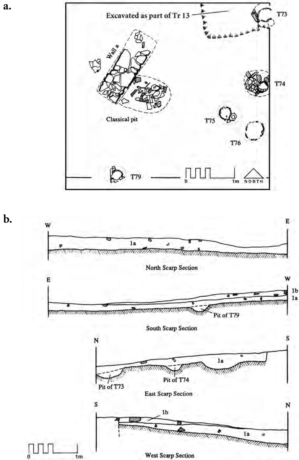
FIGURE 40. Trench 46. (a) Plan. (b) Sections.
