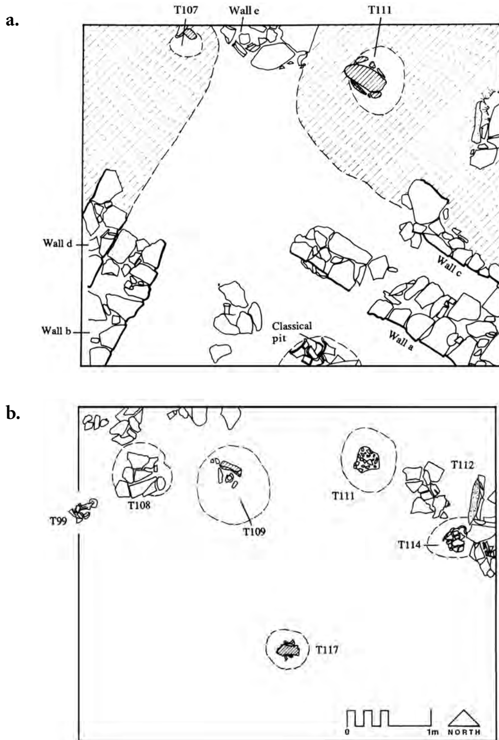
FIGURE 29 Trench 22 (on following page). (a) Plan (Stage 1). (b) Plan (Stage 2).
