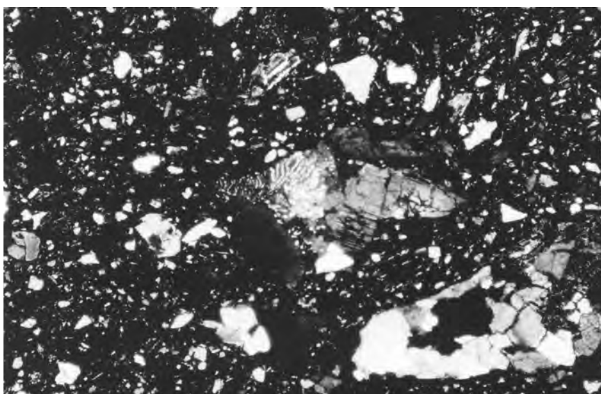
PLATE 528. Microstructure of kiln brick. Granodiorite fabric with coarse-grained inclusions, but with more micaceous (biotite) clay matrix. Width of photograph is 3.2mm.
