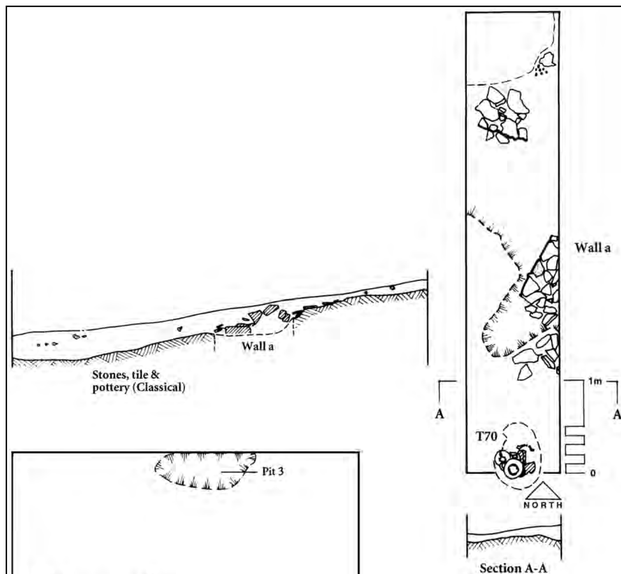
(Above): FIGURE 27. Trench 13 East Baulk. Plan and section.
