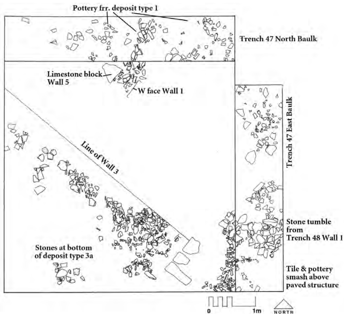
FIGURE 42. Trenches 47 and 47 North and East Baulks. Plan (Stage 1).
