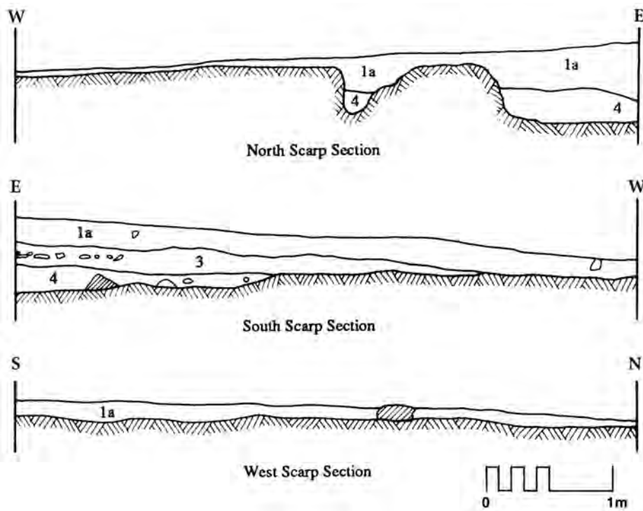
FIGURE 37 (on following page). Trench 40. (a) Plan (b) Sections.
