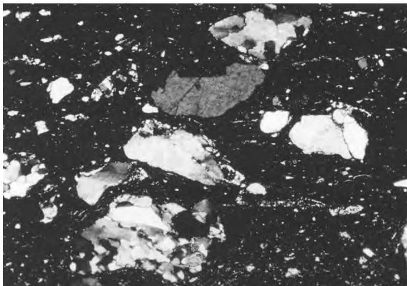
PLATE 529. Microstructure of 82.1188 ( KP-5 ). Granodiorite fabric with coarse-grained inclusions; presence of quartz-muscovite schist, a distinct bimodal grain-size distribution, and a relatively fine-grained clay matrix. Width of photograph is 3.2mm.
