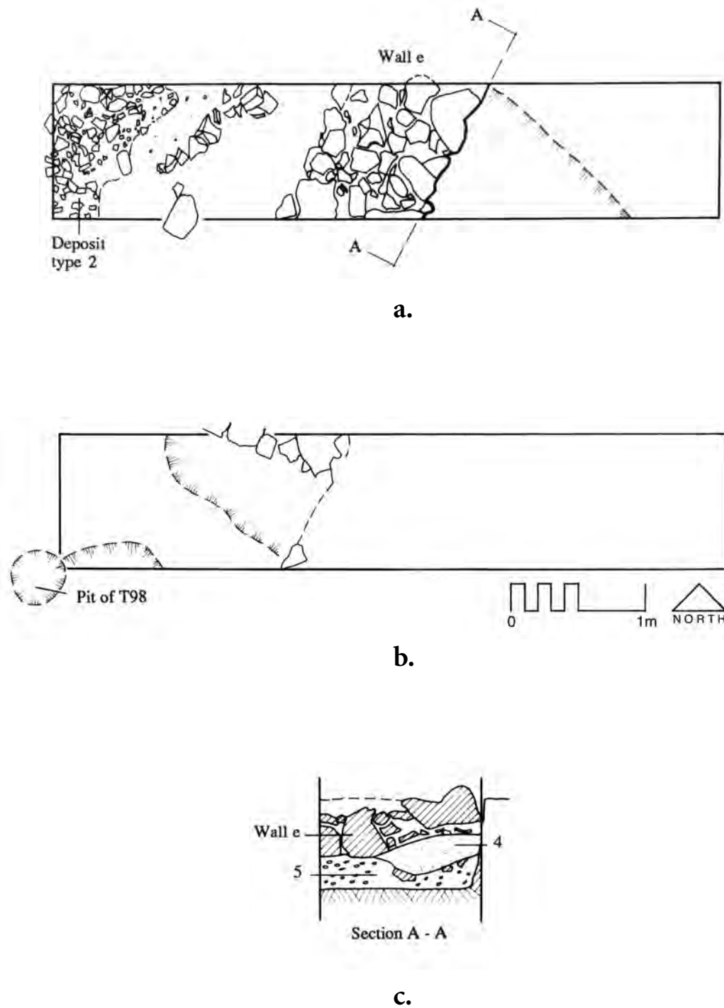
FIGURE 30. Trench 22 North Baulk. (a) Plan (Stage 1). (b) Plan (Stage 2). (c) Section.
