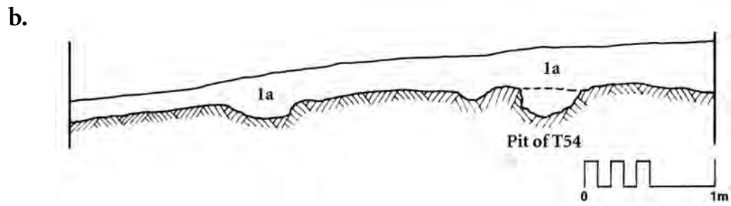
FIGURE 21 (continued). Trench 6. (b) East scarp section.
