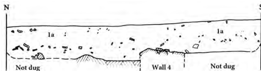
FIGURE 46. Trench 48. Section (east scarp).
