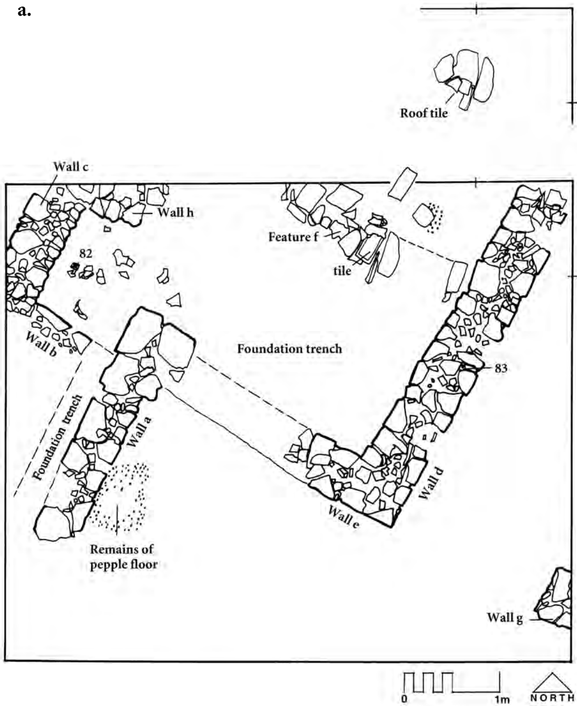
FIGURE 38 (on pages 759–761). Trench 43. (a) Plan (Stage 1), showing later phases of Classical domestic architecture and locations of Early Iron Age loomweights (82, 83).
