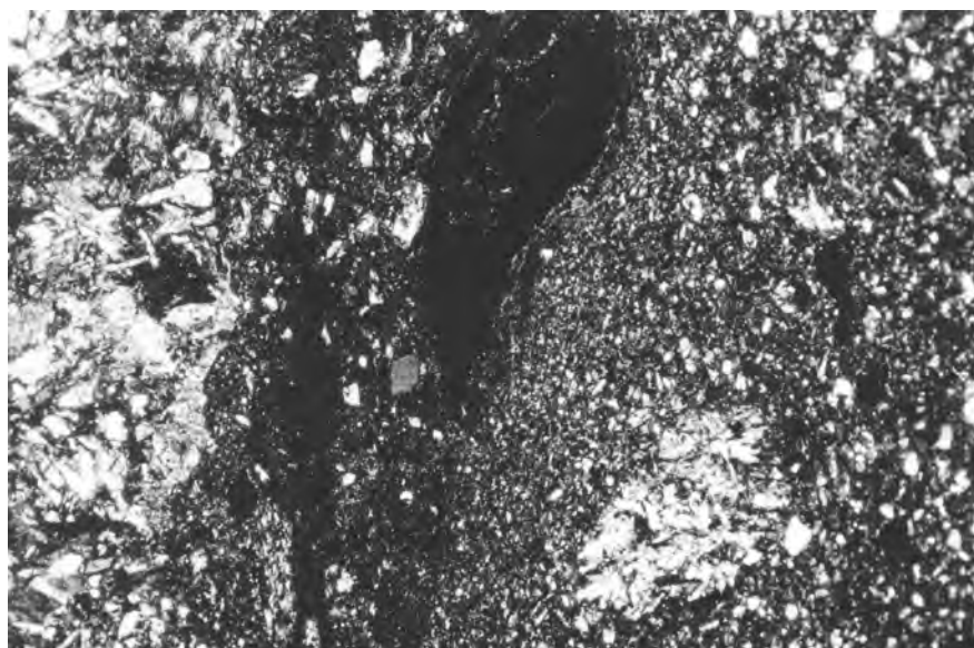
PLATE 539. Microstructure of clay sample C6, from area of amphibolite schists at the base of the NE slope of Vigla (Hill 1); fired at 900°C. Width of photograph is 3.2mm.
