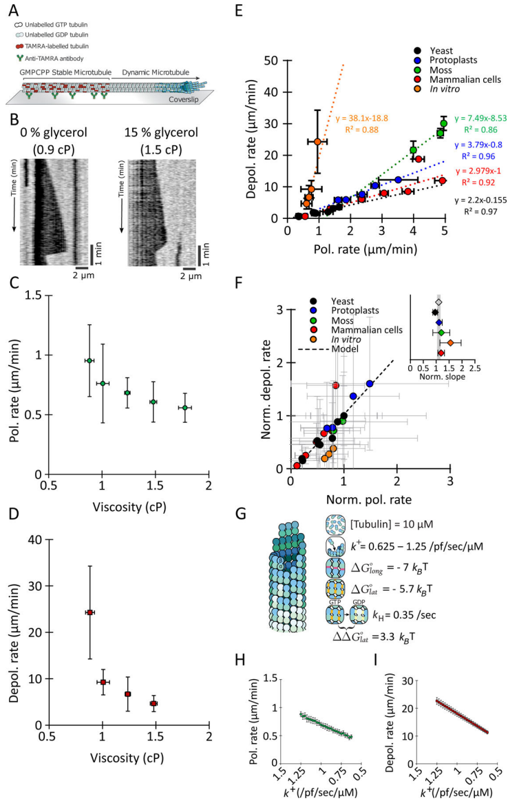
Figure 7: Increasing viscosity dampens rates of MT polymerization and depolymerization similarly.
