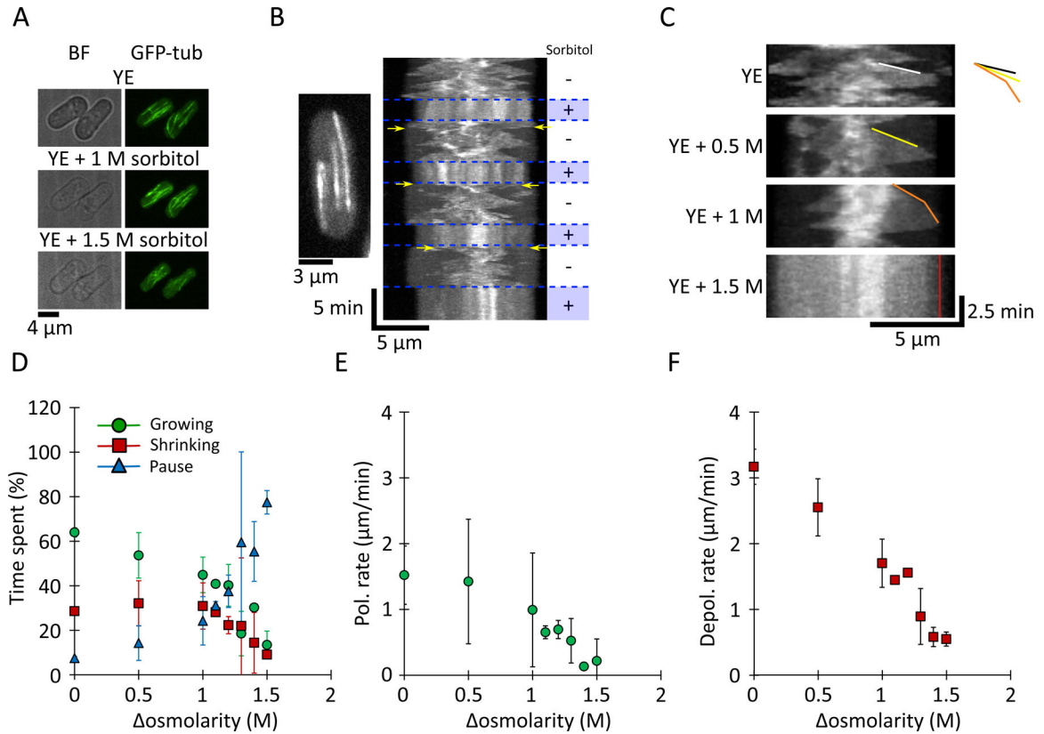
Figure 1: MT growth and shrinkage rates decrease upon hyperosmotic shock in yeast cells.
