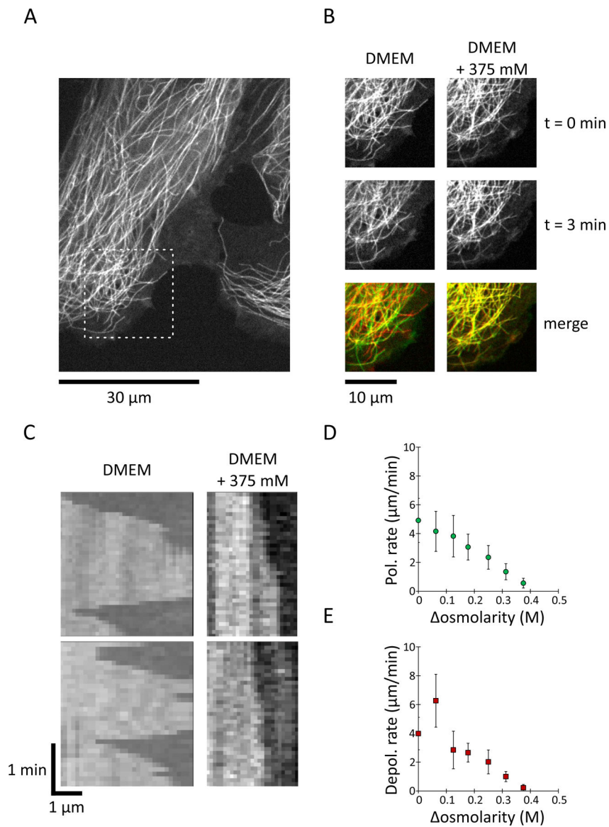
Figure 3: MT growth and shrinkage rates decrease upon hyperosmotic shock in mammalian cells.
