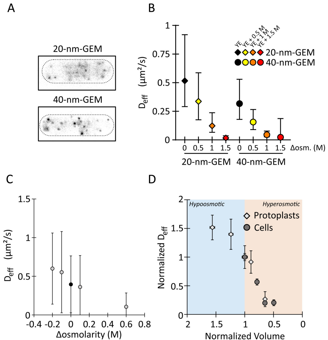
Figure 4: Nanoparticle's diffusion rate scales with cytoplasm concentration.
