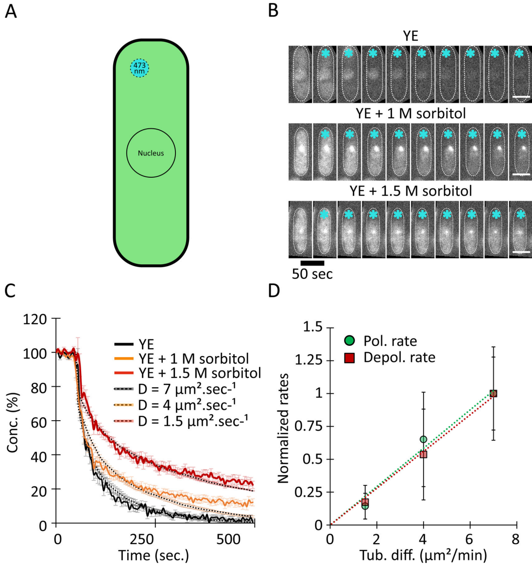
Figure 5: Hyperosmotic shifts decrease the diffusion rate of soluble tubulin.
