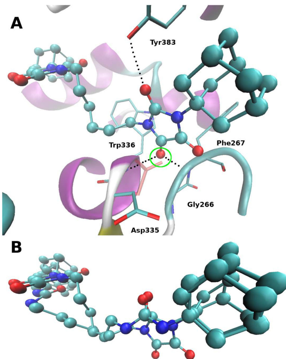
Figure 2. (A) The binding mode of the compound 2a . Black points show the hydrogen bonds which compound 2a maintain with protein residues. The green circle labels atoms which are in close proximity to each other. (B) The superposition of the docked structured of 2a and its urea derivative in the binding site.
