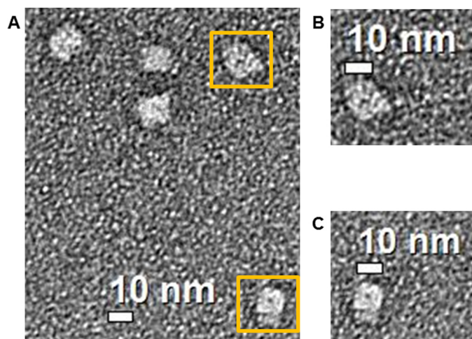
FIGURE 4. Electron microscopy analysis of the Stt7 tetramer. Diluted Stt7 (2 μg/ml) was adsorbed on a carbon-coated 400-mesh copper grid and stained with uranyl acetate. Images were recorded on an FEI Tecnai transmission electron microscope operated at 200 kV at a magnification of ×71,000 and defocus of −1 μm. A , the 2D image shows a square-like organization of the Stt7 tetramer of ~10 × 10 nm with an ~14-nm diagonal length. B and C , magnified views of two tetramers of Stt7 highlighted in A with yellow boxes. The tetramers show a dark circular feature at the center that represents a hollow cavity of ~1 nm diameter.
