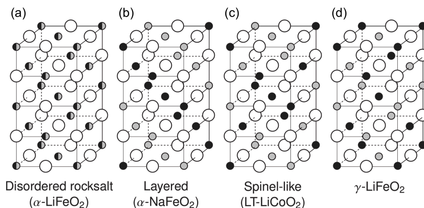
Figure 1. Common rocksalt-type lithium transition metal oxide crystal structures: (a) the disordered rocksalt \alpha - \text{LiFeO}_2 structure in which all cation sites are equivalent, (b) the layered \alpha - \text{NaFeO}_2 structure, (c) the spinel-like low-temperature \text{LiCoO}_2 structure, (d) the \gamma - \text{LiFeO}_2 structure. Large empty circles indicate oxygen sites, small gray and black filled circles stand for lithium and transition metal sites, respectively. Adapted with permission from Urban et al. 22 Copyright Wiley-VCH.
