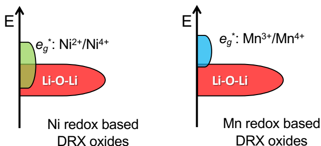
Figure 14. Qualitative diagrams of transition metal and oxygen electronic states in \text{Ni}^{2+}/\text{Ni}^{4+} redox-based and \text{Mn}^{3+}/\text{Mn}^{4+} redox-based DRXs.
