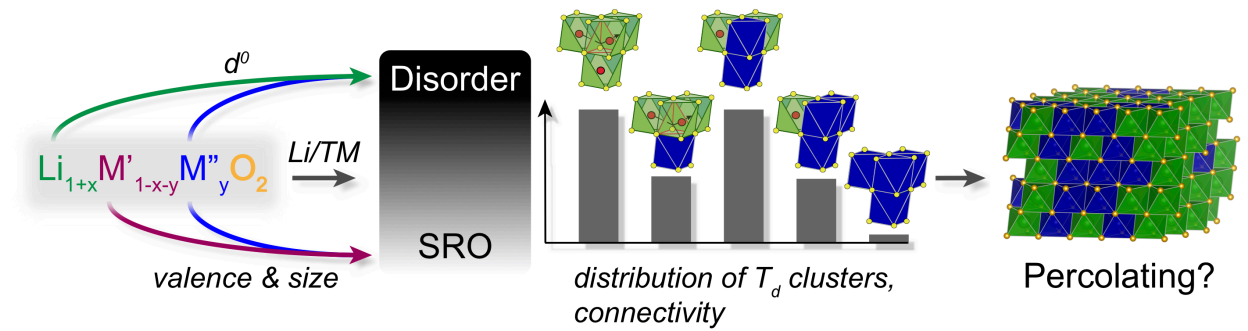
Figure 9. Factors contributing to the stabilization of a DRX lithium transition metal oxide structure, and to the \text{Li}^+ transport properties of the electrode material.
