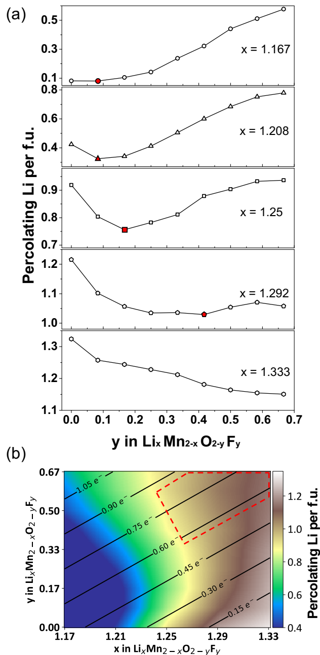
Figure 12. (a) Li percolation in \text{Li}_x \text{Mn}_{2-x} \text{O}_{2-y} \text{F}_y DRX cathodes as a function of F (y values) at various Li-excess levels (x values). For each Li excess level, the critical F content at which Li percolation encounters a minimum is highlighted in red. (b) Design map within the Li-Mn-O-F DRX space. The color scale represents the total amount of percolating Li per formula unit (f.u.) through the 0-TM percolation network at each composition, obtained from Monte Carlo simulations at 2573 K. The solid lines and numbers in this map indicate the theoretical Mn redox capacity. The region of compositional space where DRX Li-Mn-O-F cathodes with a high capacity and good cyclability are likely to be obtained is enclosed with a red dashed line. Adapted from Chem, in press , Z. Lun, B. Ouyang, Z. Cai, R. J. Clément, D.-H. Kwon, J. Huang, J. K. Papp, M. Balasubramanian, Y. Tian, B. D. McCloskey, H. Ji, H. Kim, D. A. Kitchaev, G. Ceder, Design
