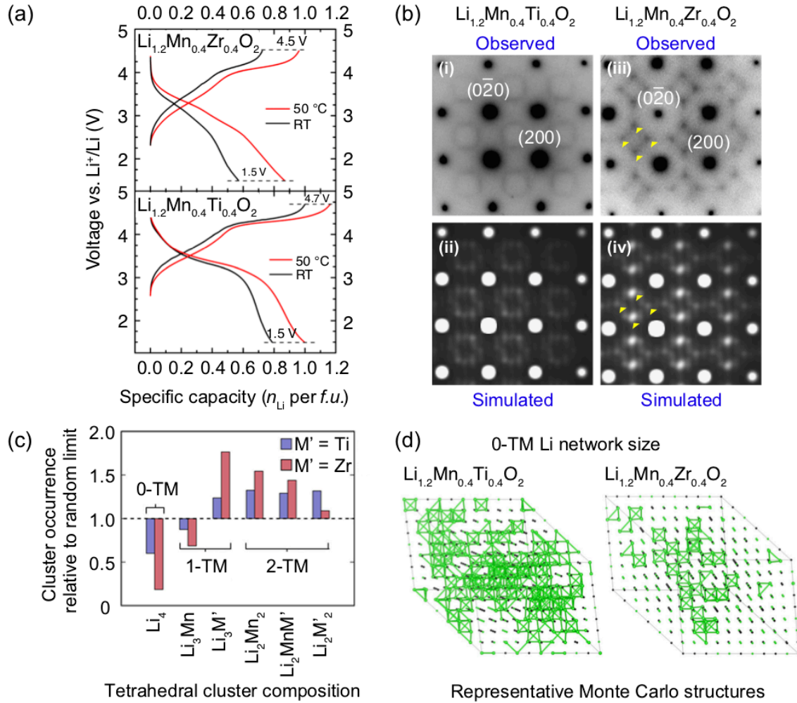
Figure 8. (a) Comparison of room temperature and 50°C galvanostatic cycling data for \text{Li}_{1.2}\text{Mn}_{0.4}\text{Zr}_{0.4}\text{O}_2 (top panel) and \text{Li}_{1.2}\text{Mn}_{0.4}\text{Ti}_{0.4}\text{O}_2 (bottom panel). (b) Electron diffraction patterns of (i) \text{Li}_{1.2}\text{Mn}_{0.4}\text{Ti}_{0.4}\text{O}_2 and (iii) \text{Li}_{1.2}\text{Mn}_{0.4}\text{Zr}_{0.4}\text{O}_2 along the [100] zone axis. The round spots are indexed to the Fm\bar{3}m space group, while the diffuse scattering patterns around the spots are attributed to SRO. Several intensity maxima in the diffuse scattering pattern of \text{Li}_{1.2}\text{Mn}_{0.4}\text{Zr}_{0.4}\text{O}_2 are highlighted with yellow arrows. Simulations of electron diffraction patterns for (ii) \text{Li}_{1.2}\text{Mn}_{0.4}\text{Ti}_{0.4}\text{O}_2 and (iv) \text{Li}_{1.2}\text{Mn}_{0.4}\text{Zr}_{0.4}\text{O}_2 along the same zone axis are consistent with experimental observations. (c) Occurrence of various tetrahedron clusters (0-TM, 1-TM, 2-TM) in \text{Li}_{1.2}\text{Mn}_{0.4}\text{Ti}_{0.4}\text{O}_2 (blue) and \text{Li}_{1.2}\text{Mn}_{0.4}\text{Zr}_{0.4}\text{O}_2 (red), as compared to the random limit (dotted line). The analysis is based on structures derived from Monte Carlo simulations at 1000°C. (d) Representative Monte Carlo structures for \text{Li}_{1.2}\text{Mn}_{0.4}\text{Ti}_{0.4}\text{O}_2 and \text{Li}_{1.2}\text{Mn}_{0.4}\text{Zr}_{0.4}\text{O}_2 . \text{Li}^+ ions are labeled with green spheres and 0-TM connected Li sites are bridged with green bonds. 21 Figures adapted from Ji et al. 21 under the Creative Commons CC BY license.
