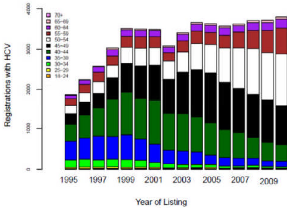
Figure 2. HCV + by listing year and age at listing for liver transplantation
