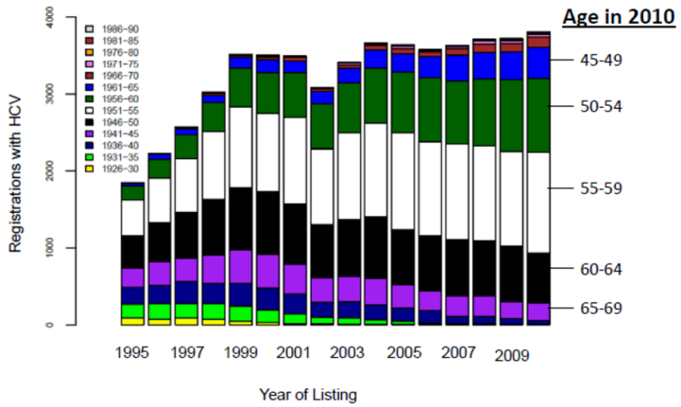
Figure 3. All new registrants for liver transplantation with HCV by listing year and birth cohort
