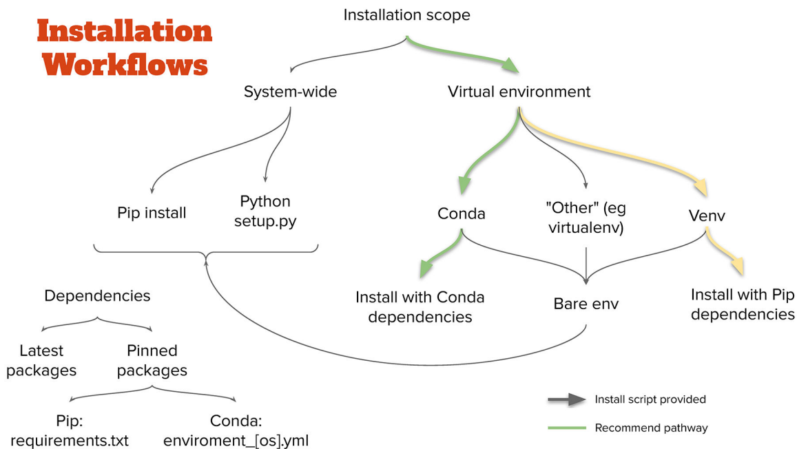
Figure 2. Installation pathways. As with many Python applications, MagellanMapper can be installed through several pathways. The recommended pathway is through Conda, which handles all required dependencies and keeps them separate from any other installed Python packages in a virtual environment. For those who prefer a more “pure Python” approach, Venv will also keep packages separate in an environment while installing dependencies through Pip. Installation scripts are provided to simplify the Conda pathway. Various other pathways are also available. Typically, the latest dependencies are installed, but specifications that pin each dependency version are available for reproducibility.
