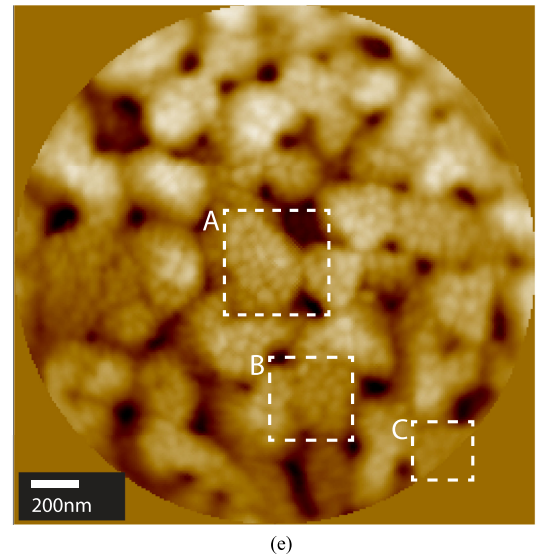
Fig. 3. CAV spiral. (a) Velocity as a function of scan time increases linearly and (b) angular frequency is constant. (c) Theoretical data density is very high in the center and getting sparse toward the periphery. (d) The velocity is low in the middle and high on the periphery. (e) CAV image of copper evaporated onto annealed gold at same location as Fig. 2. The CAV eliminates errors in the center of the image but the high linear velocity and sparse data at the edges smears out features. The features in the boxes are compared with other scan waveforms in Fig. 5.
