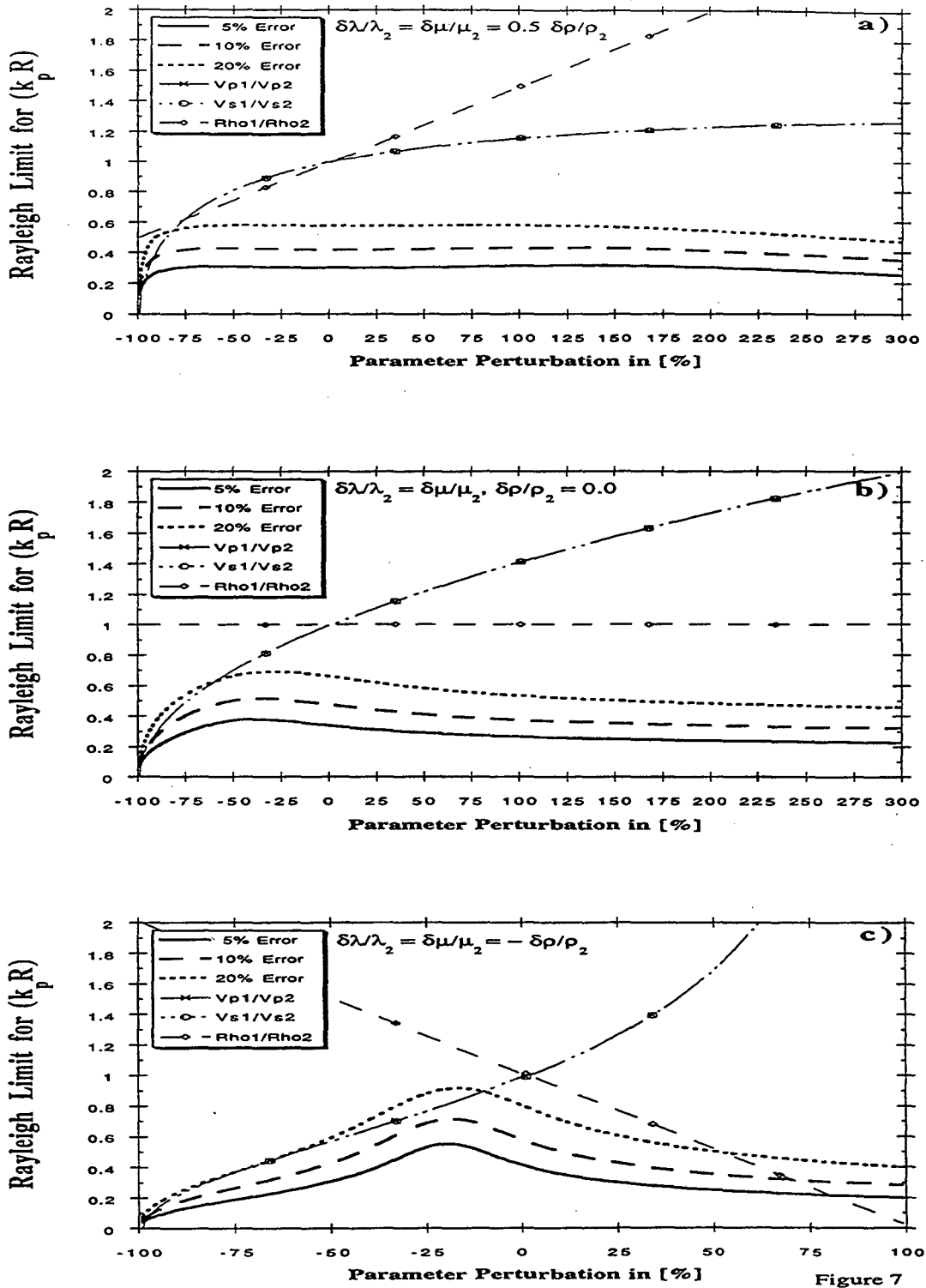
Figure 7 Rayleigh limit for the parameter k_p R as a function of parameter perturbation. The three curves correspond to three investigated error limits of 5%, 10% and 20%. Also plotted are the velocity and density ratios associated with the chosen relation between the elastic parameters.
