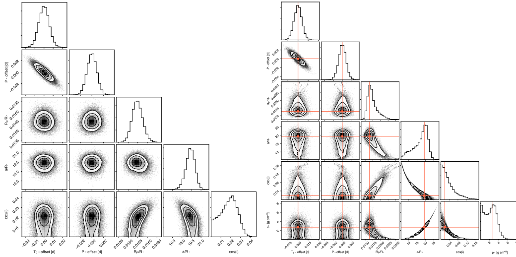
Figure 5. Same as Figure 4 for planet c.
