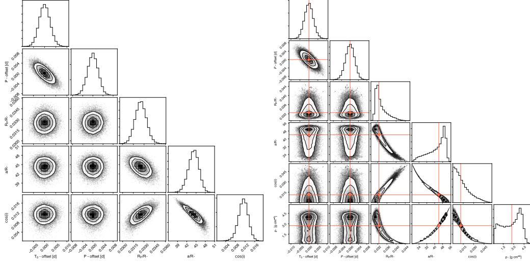
Figure 6. Same as Figure 4 for planet d.
