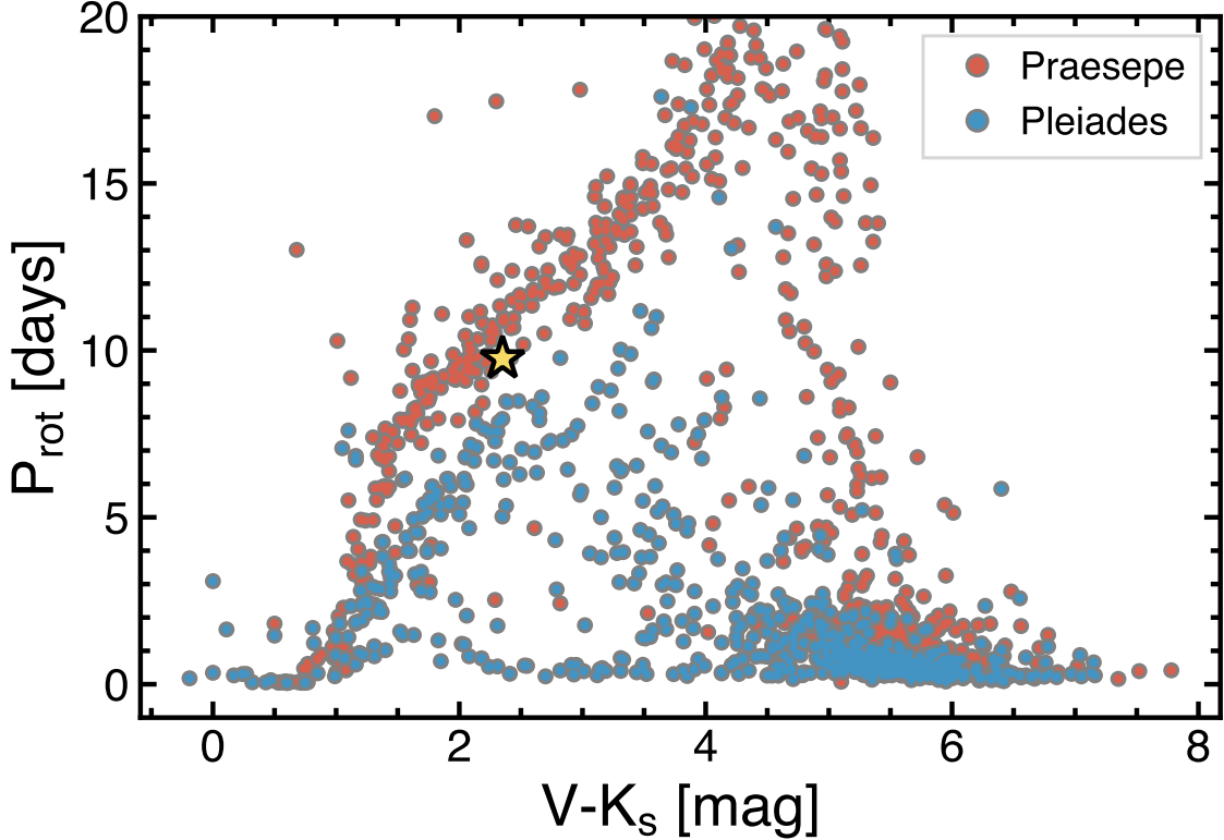
Figure 2. Period-color diagram for open cluster members observed by K2 (Rebull et al. 2016, 2017) and K2-233 (gold star).
