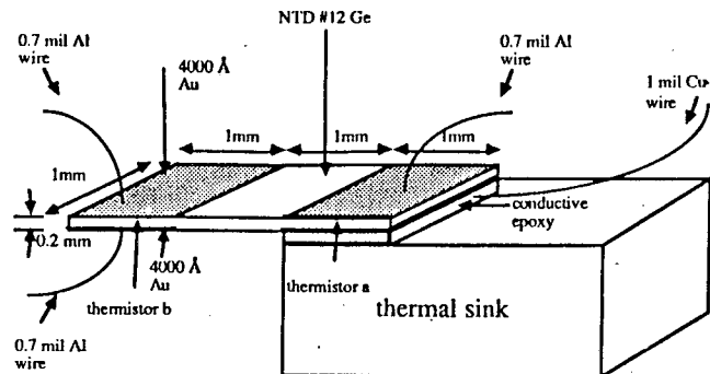
Figure 1. Schematic diagram showing the configuration of the thermally clamped double thermistor. The entire Ge chip is uniformly doped by neutron transmutation.
