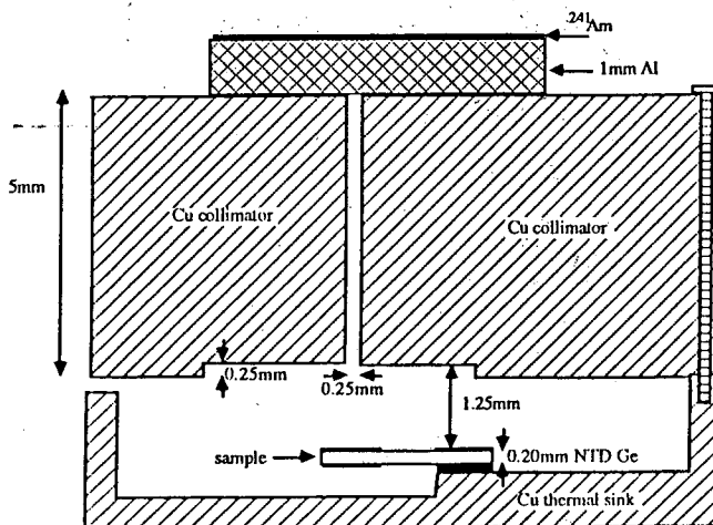
Figure 2. Arrangement for collimating the 241 Am X-rays onto thermistor a.
