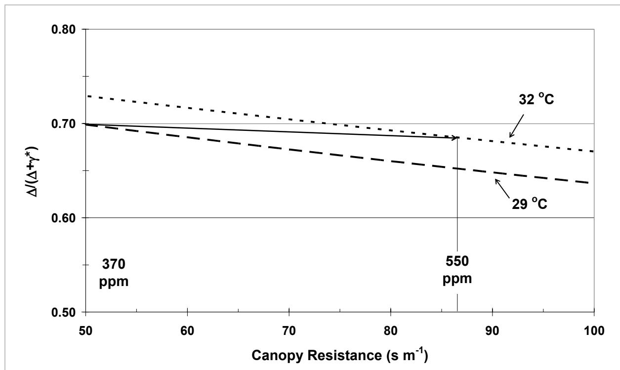
Figure 7-15. A plot of \Delta/(\Delta + \gamma^*) versus canopy resistance for a 3^\circ\text{C} temperature increase as a function of canopy resistance.
