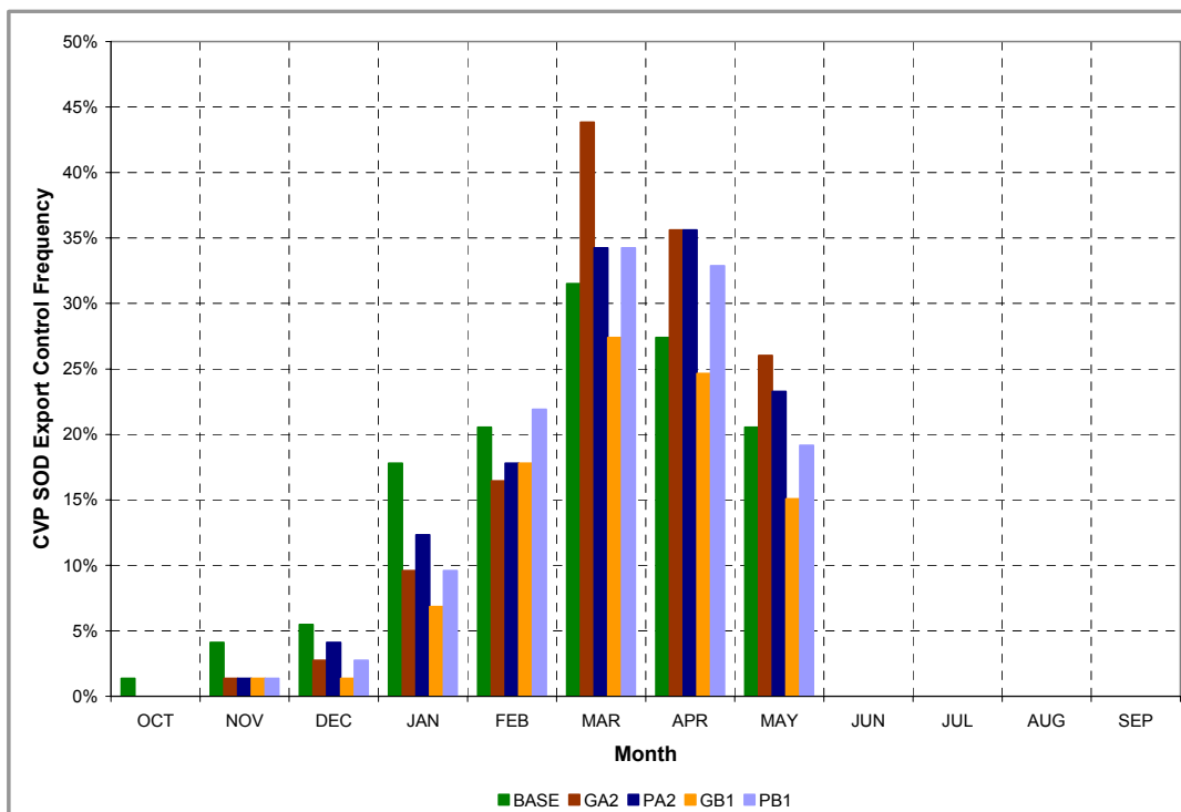
Figure 4.29 Operational control frequency of CVP SOD conveyance capacity on Tracy exports
