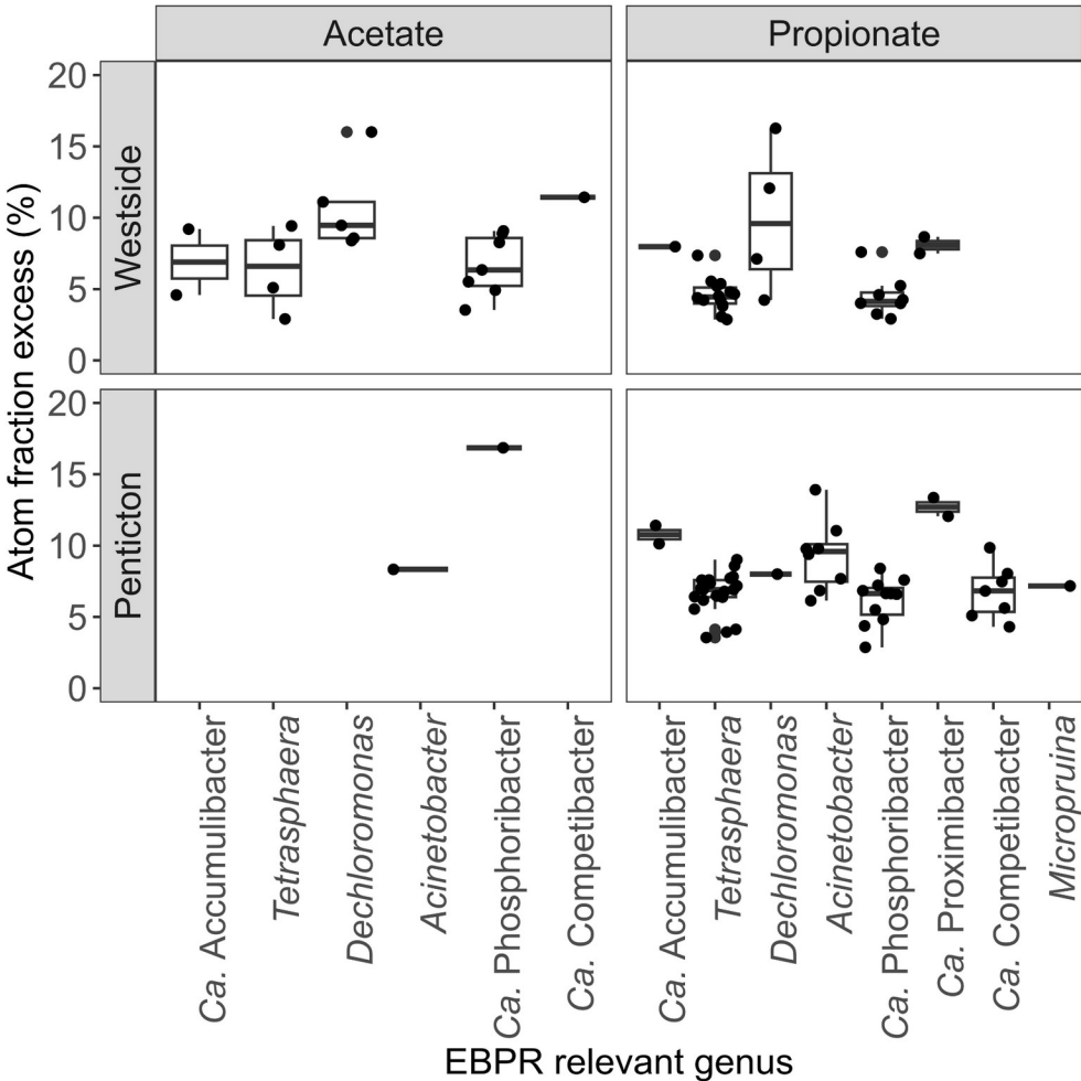
321 Figure 2. Atom fraction excess (AFE) of active EBPR-relevant 16S rRNA ASVs in the four SIP 322 incubations. Boxplots indicate the distribution of AFEs for the ASVs within the same genera, and 323 the points indicate the lower bounds of the FCR adjusted 95% confidence interval of bootstrapped 324 (10,000 times) AFEs.
