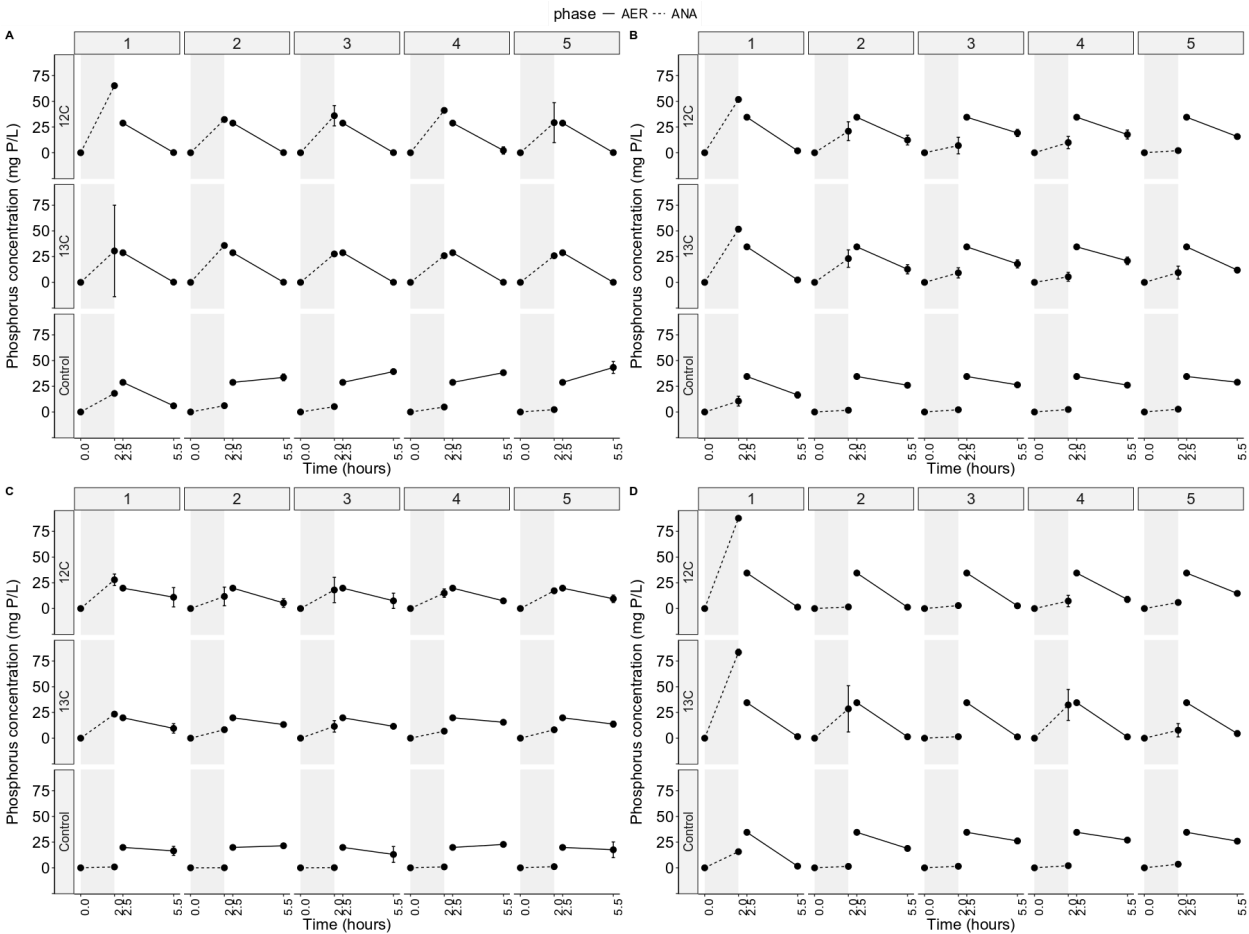
272 Figure 1. P dynamics in the five aerobic (light shade; ‘AER’) and anaerobic (dark shade; ‘ANA’) 273 phases in the 12 C, 13 C, and control triplicates from the (A) ‘Westside+acetate’, (B) 274 ‘Westside+propionate’, (C) ‘Penticton+acetate’, and (D) ‘Penticton+propionate’ SIP incubations. 275 Half-hour gaps in the timeline indicate the wash step between phases. P concentrations in the
