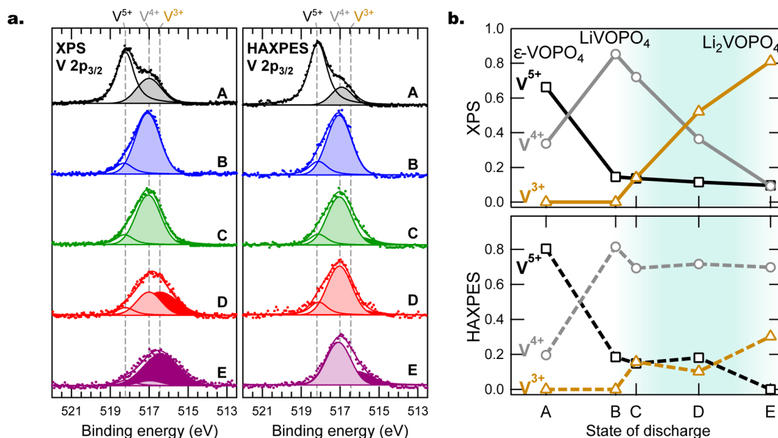
Figure 4. (a) Peak fitting of the V 2p_{3/2} core level obtained from XPS (left) and HAXPES (right) for electrodes A–E along the first discharge curve scaled such that the total area under each curve is equal to 1. (b) Vanadium oxidation state ratios obtained from peak fitting XPS (top) and HAXPES (bottom) spectra for increasing depth of discharge.
