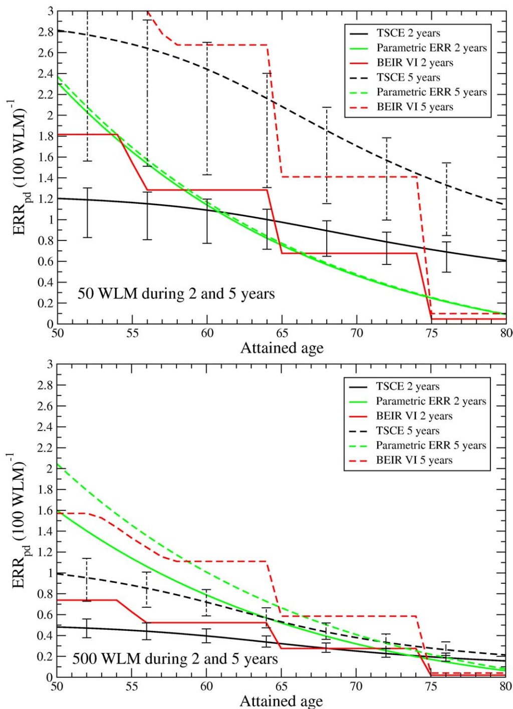
Figure 4. ERR pd for persons with total RDP exposure of 50 and 500 WLM. The exposures were received around age 30 for durations of 2 and 5 years, the 68% uncertainty bounds for the TSCE model are shown. doi:10.1371/journal.pone.0041431.g004
