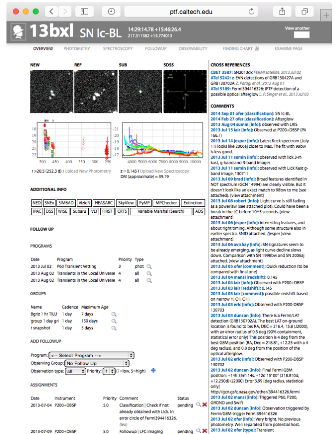
Figure 13. Screenshot of the iPTF Transient Marshal, showing GRB 130702A / iPTF13bx1.
