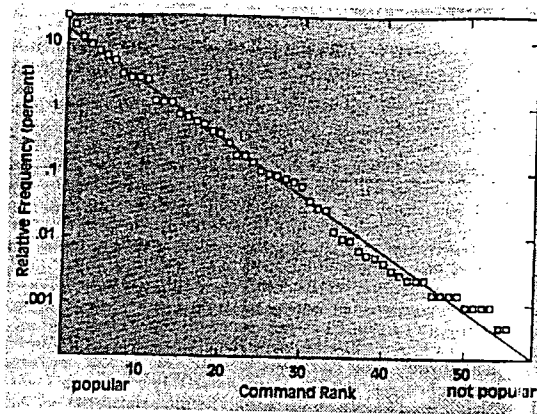
Figure 14. Relative command frequencies ordered by "rank".
