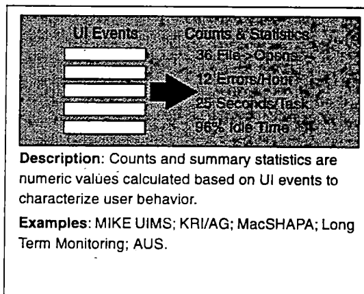
Figure 6. Counts and Summary Statistics
