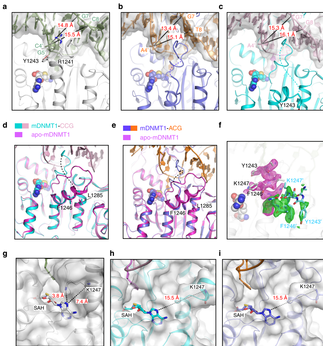
Fig. 5 Conformational transition of the catalytic helix of murine DNMT1. Close-up views of the conformation of the catalytic helix in the GCG (PDB 4DA4) ( a ), ACG ( b ), and CCG ( c ) complexes. The side chains of the DNA-interacting residues R1241 and Y1243 are shown in stick representation in the GCG complex ( a ). These two residues are either completely (in the ACG complex) or partially (CCG complex) non-traceable in the other two complexes. The hydrogen-bonding interaction is shown as dashed line in red. The minor groove width at the +2 flank sites (C4'/A4') is indicated by dashed lines in black. The disordered segments in ( b ) and ( c ) are shown by dashed lines in slate and cyan, respectively. Close-up view of the catalytic helix overlaid between a DNMT1 structure with no DNA bound to the catalytic domain (PDB 3PT9) and the CCG complex ( d ) or the ACG complex ( e ). Fo-Fc omit map of residues 1242-1249 of mDNMT1 731-1602 in the GCG DNA complex (PDB 4DA4). The straight conformation and associated map (2.0 \sigma level) are colored in silver and magenta, respectively. The kinked conformation and associated map (1.9 \sigma level) are colored in aquamarine and green, respectively. Enlargement of the AdoMet-binding pockets in the GCG ( g ), CCG ( h ) and ACG ( i ) complexes. The distances between the N7 atom of AdoMet (SAH) and the side chain or the backbone of residue K1247 are indicated by dashed lines. Note that the side chain of K1247 is non-traceable in ( h-i ) due to missing electron density.
