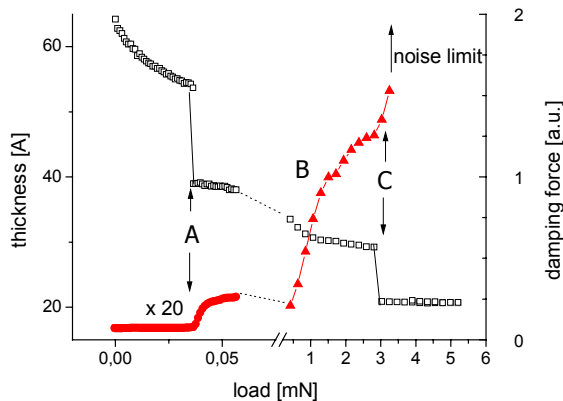
Fig. 5. Damping force (triangles) and film thickness (squares) for octanol subjected to shear between mica surfaces vs. applied load. The damping force is proportional to the viscosity. Symbols A, B and C indicate the corresponding states in Fig. 1. In region B the separation between mica surfaces remains constant but the area of the contact increases. The damping force at low loads is shown magnified 20 times. Notice the change in the load scale in region B.
