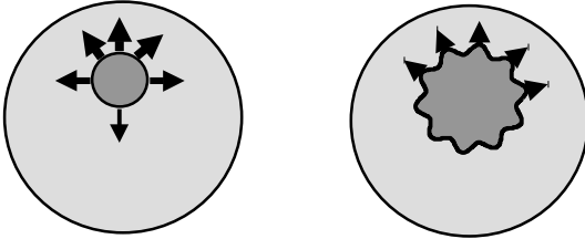
Fig. 7. a) Schematic of an off-center hole (dark area). The two-dimensional pressure gradient between the boundary of the hole and the edge of the contact is steepest where their separation is minimal, leading to a larger flow velocity, as indicated by the arrows. b) Same situation as in a), for a hole with a perturbed boundary. Arrows indicate how the differences in pressure gradient let the perturbation increase with time.
