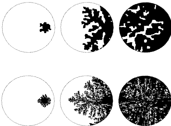
Fig. 8. Snapshot of the layering transition in the kinetic Monte Carlo simulation. Top: with and bottom: without line tension. To calculate the P_{2D} , a radial pressure distribution according to Hertzian contact theory was used.
