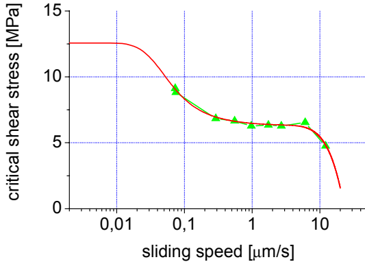
Fig. 4. Critical shear stress vs. sliding speed at F_N = 8.8 mN. The solid line is a fit according to eq. (5) in the text, which describes the exponential growth of interdigitation or, in our case crystallographically locked domains.
