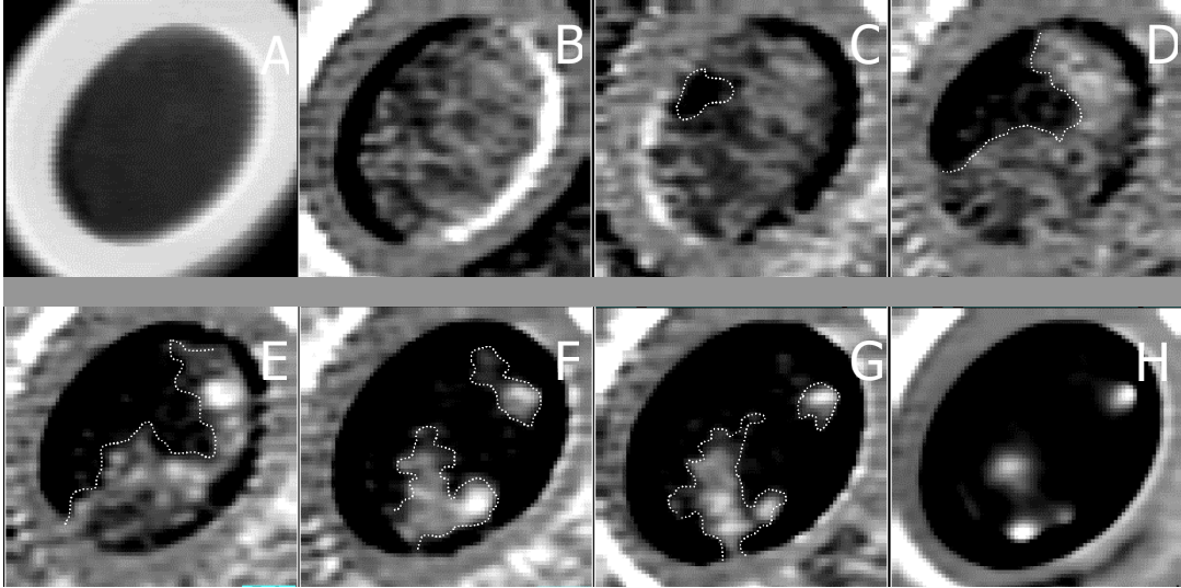
Fig. 6. Snapshots of the contact area during the layering transition ( 100\ \mu\text{m} \times 100\ \mu\text{m} size). The initial (A) and final state (H) images are averaged for noise reduction. Images B to H are difference images with the initial state (A). Images B to G are recorded at 0.16 sec time intervals. Darker color corresponds to smaller film thickness. The dark and bright rim at the edge of the contact area in B and C are artifacts related to the subtracting of video images.
