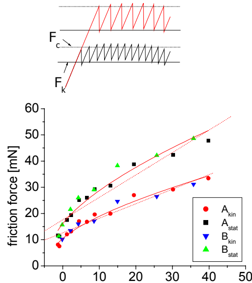
Fig. 2. Critical and kinetic friction force vs. load at a constant sliding speed of 1 \mu\text{m/s} for \text{C}_{11}\text{OH} . A and B correspond to independent experiments. Dotted lines are linear fits and solid lines are curves fitting the JKR model. Top: Shear force vs. time for stick-slip friction at two different loads.
