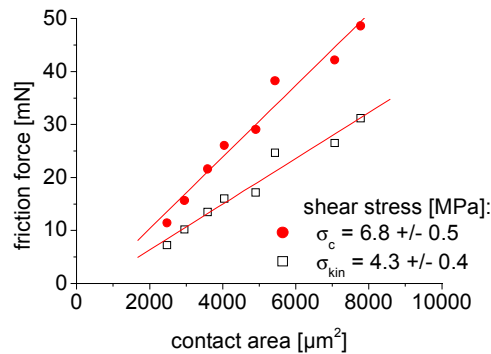
Fig. 3. Critical and kinetic friction force vs. the measured contact area (same friction data as in Fig.
