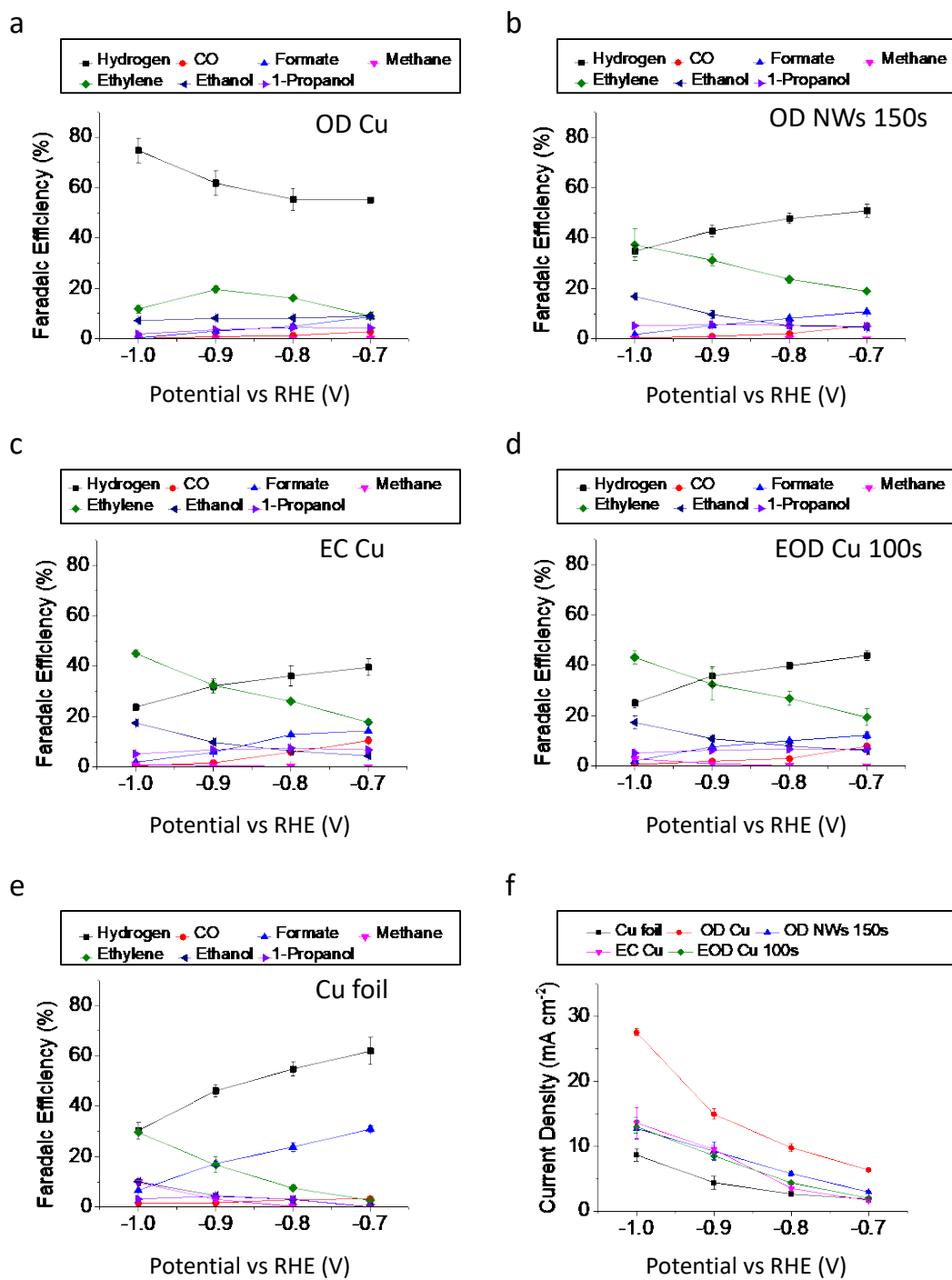
Figure 3 Faradaic efficiencies of major CO 2 R products from -0.7 V to -1.0 V vs RHE in 0.1 M CsHCO 3 for: (a) OD Cu; (b) OD NWs 150s; (c) EC Cu, (d) EOD Cu 100s and (e) Cu foil.
