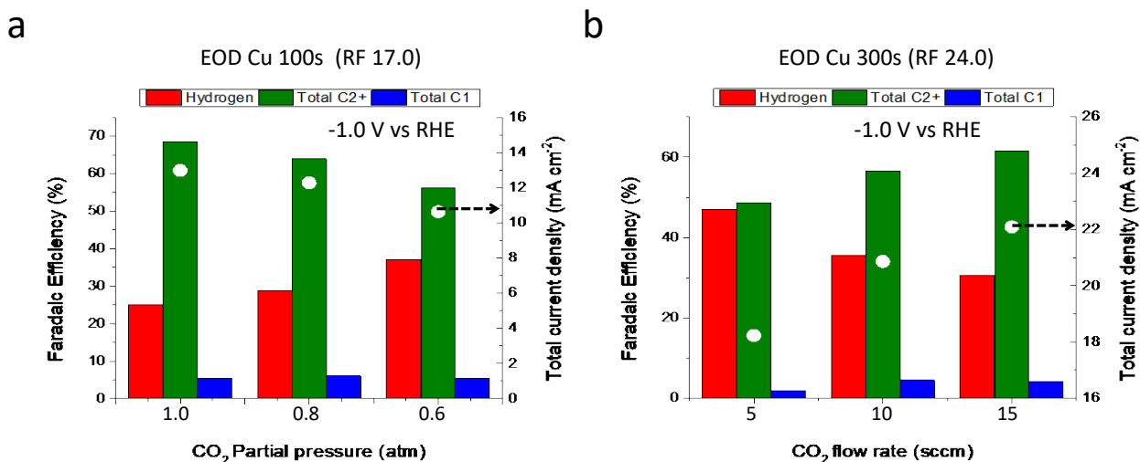
Figure 5 Faradaic efficiencies and partial current densities towards H 2 , C 2+ products and C 1 products at -1.0 V vs RHE for: (a) EOD Cu 100s with different CO 2 partial pressures and (b) EOD Cu 300s with different flow rates of CO 2 . A lower CO 2 partial pressure results in a lower concentration of dissolved CO 2 , while a higher flow rate results in a smaller mass-transfer boundary layer thickness. White circles correspond to total current density values. Bar graphs correspond to faradaic efficiency values. More detailed faradaic efficiency and current density data are available in the supporting information (Table S5 and S6).
