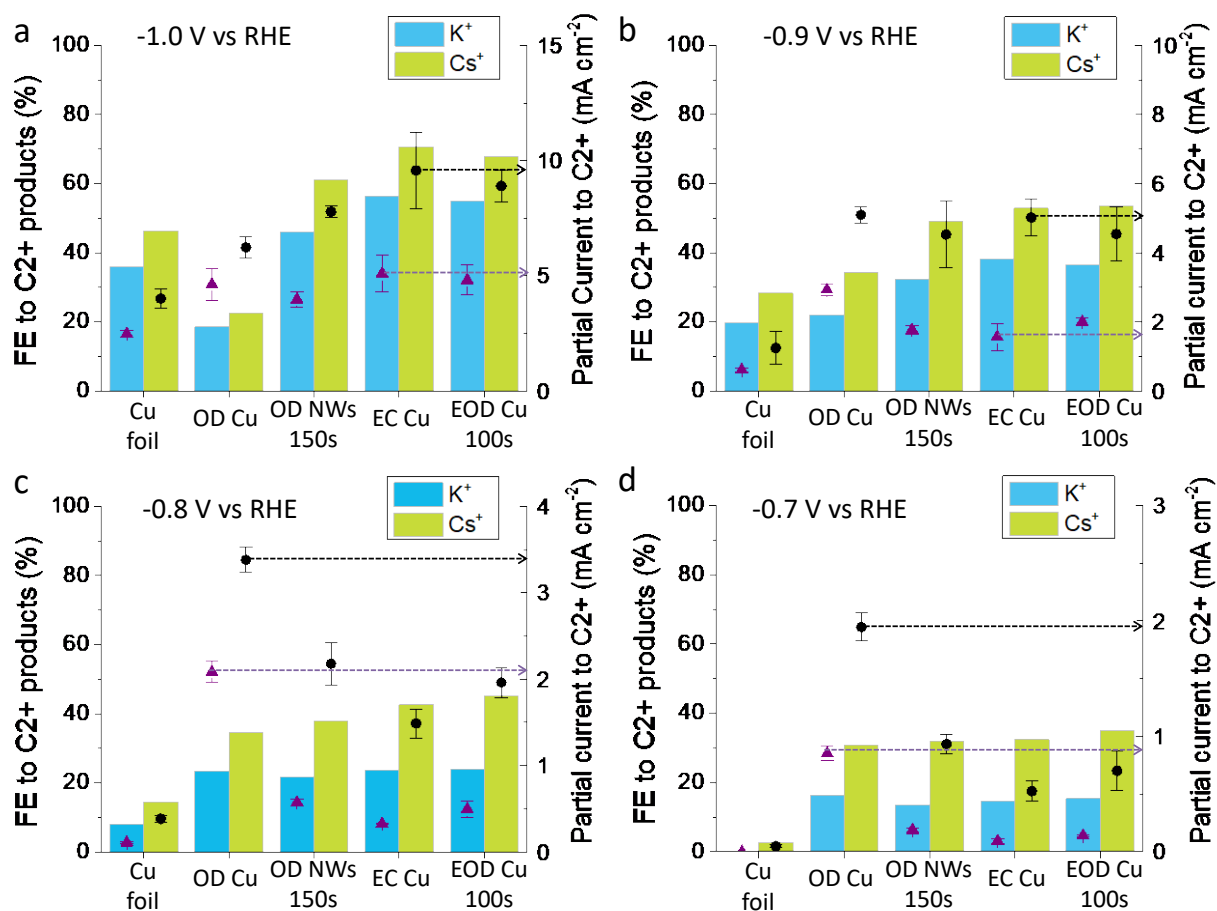
Figure 2 Faradaic efficiencies and partial current densities towards C_{2+} products for catalysts tested in both K^+ electrolyte and Cs^+ electrolyte: (a) -1.0 V vs RHE (b) -0.9 V vs RHE; (c) -0.8 V vs RHE (d) -0.7 V vs RHE. Purple triangles and black circles correspond to partial current density values to C_{2+} products for samples tested in K^+ electrolyte and Cs^+ electrolyte respectively. Bar graphs correspond to faradaic efficiency values (blue, K^+ electrolyte; green, Cs^+ electrolyte). More detailed faradaic efficiency and current density data are available in the supporting information.
