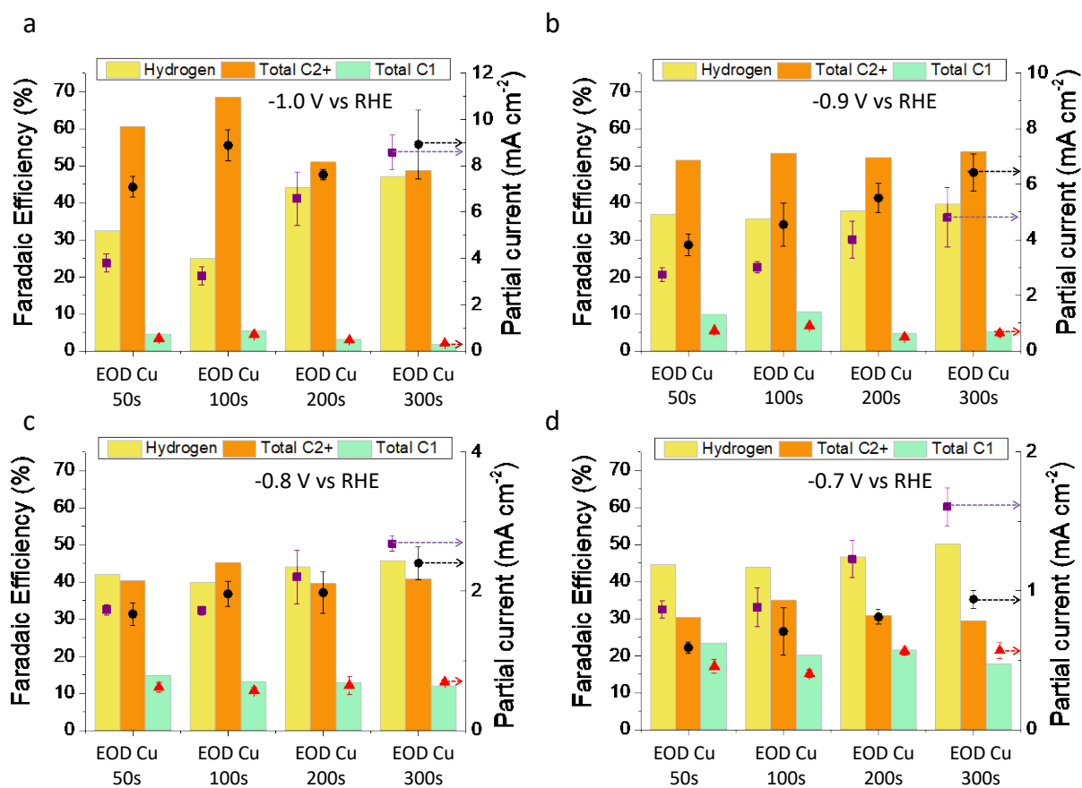
Figure 4 Faradaic efficiencies and partial current densities towards H 2 , C 2+ products and C 1 products for different thicknesses of electrodeposited Cu oxide layer tested in Cs + electrolyte at
