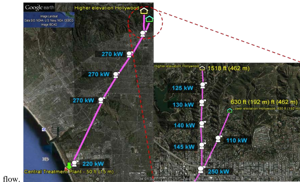
Figure 3.12 Pump-back Energy consumption for Hollywood, CA
