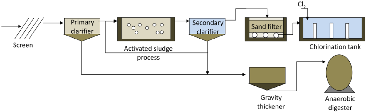
Figure 3.8 Hypothetical wastewater treatment configuration for analysis
