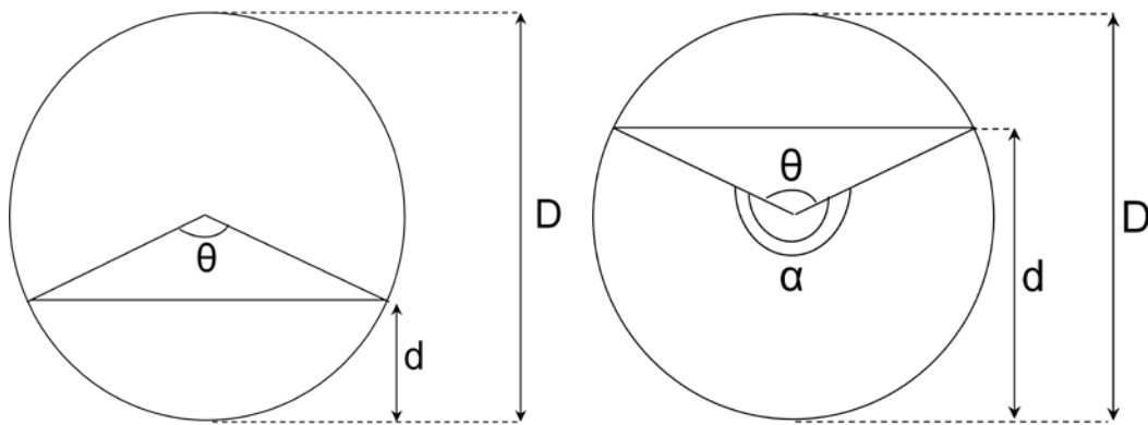
Figure 3.10 Sewer with partial flow ( d/D \leq 0.5 ) (left); Sewer with partial flow ( d/D \leq 0.5 ) (right)
