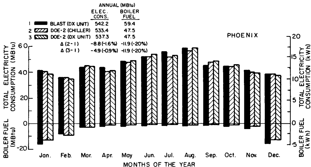
FIG. 2 SITE (BUILDING BOUNDARY) ENERGY CONSUMPTION
