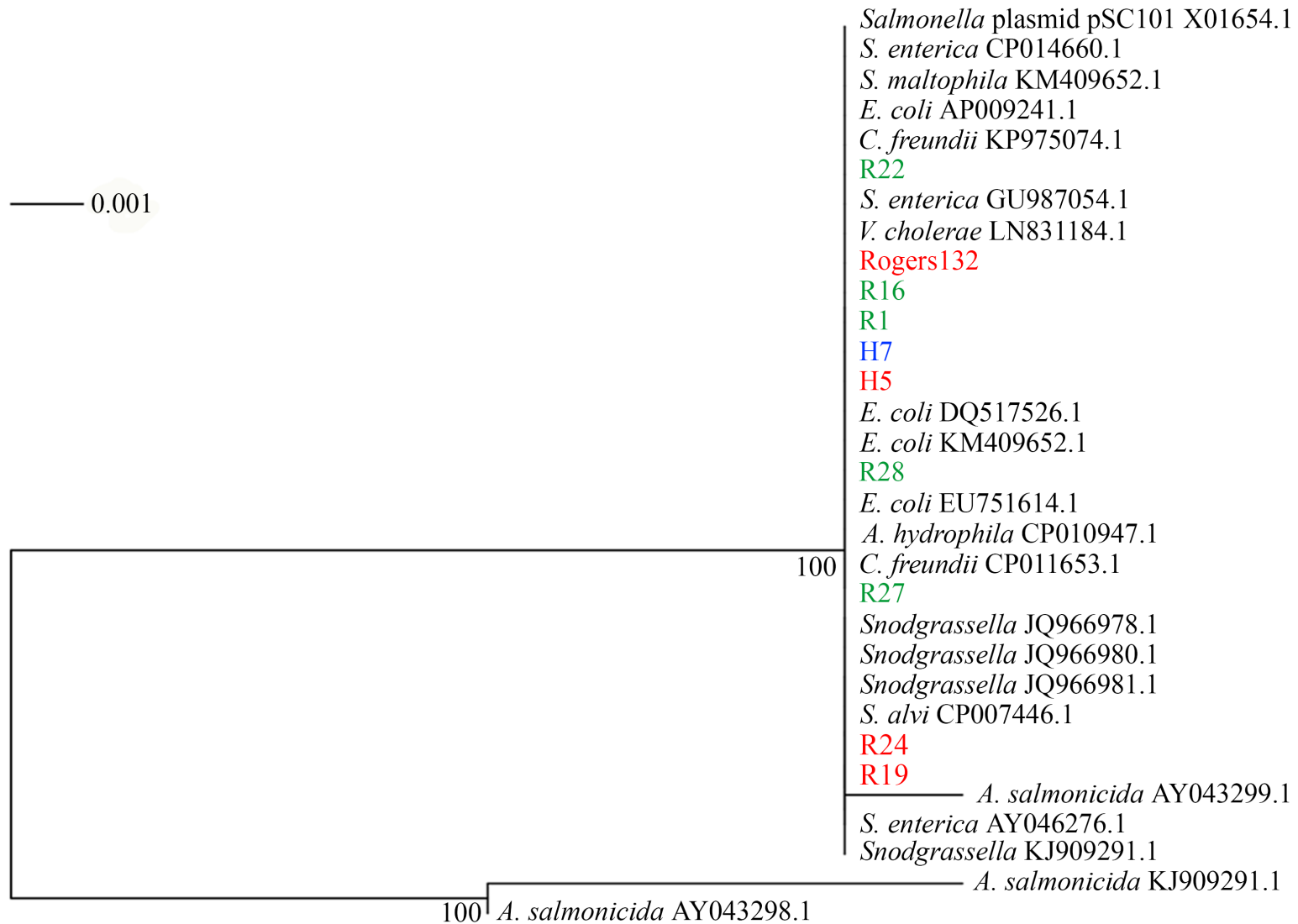
Figure S2. The tetracycline repressor gene tetR(C) is highly conserved across genera. Shown is the unrooted Maximum Likelihood (ML) phylogenetic tree of tetR(C) for a number of tetracycline resistant bacteria (NCBI, BLASTN search, identity cover: 98%) and ten C. suis strains, which correspond to two separate clades (Clade 1: red; Clade 2: green) and H7 (blue).
