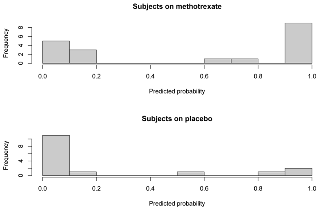
Appendix Figure 2. Histogram of the predicted probabilities of improving in subjects in the RCT study of methotrexate vs. placebo.
