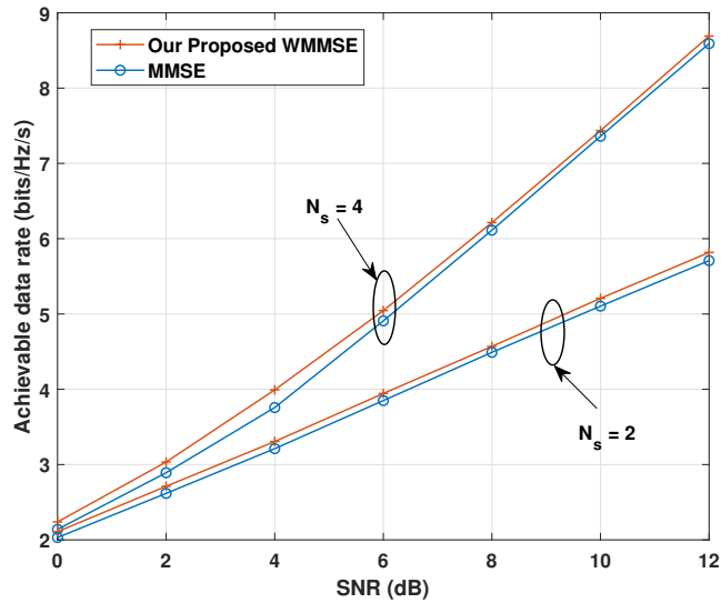
Fig. 11: Baseband algorithms comparison
