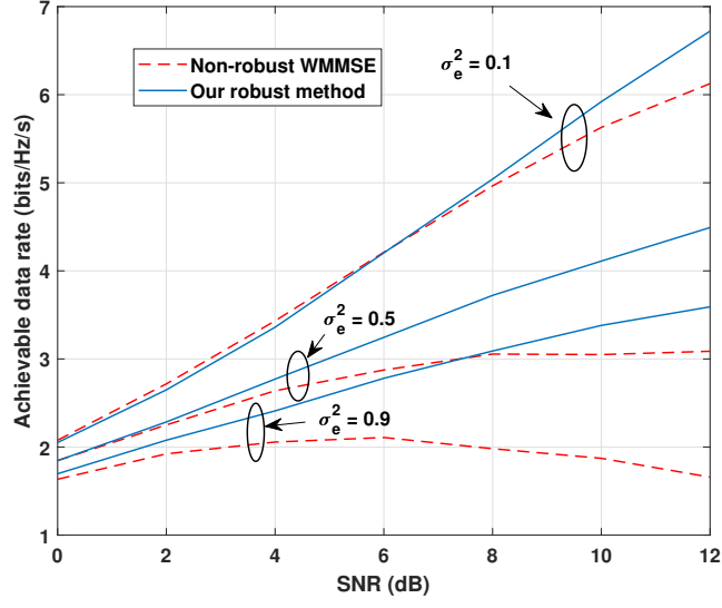
Fig. 14: Achievable rate comparison when \alpha = 0.5 , \beta = 0.5
