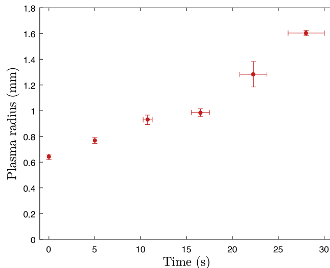
Fig. 7 Evolution of the radius of the positron plasma as a function of time during the laser cooling frequency sweep. The plasma was a mixture of 2.6 \times 10^6 e^+ and \sim 4\text{--}5 \times 10^5 Be^+ ions. Time zero is when the frequency sweep begins. The total sweep time we use to sympathetically cool the positrons to their lowest temperatures is 40 s. It is not possible to measure plasma radii greater than around 1.6 mm with our current MCP imaging diagnostic. The error corresponds to the standard error on the mean radius measured (vertical bars) and the laser-cooling time (horizontal).
