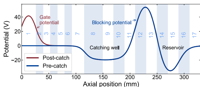
Fig. 6 Potentials on-axis for Be^+ capture and stacking. Shaded and numbered regions represent electrode positions. Ions enter from the left into the blue potential. Subsequently, the gate electrode (E1) is raised to 40 V (red potential) to capture them. Ions are then moved to the reservoir where they are combined with previous loads and laser-cooled until the desired number of stacks have been accumulated.
