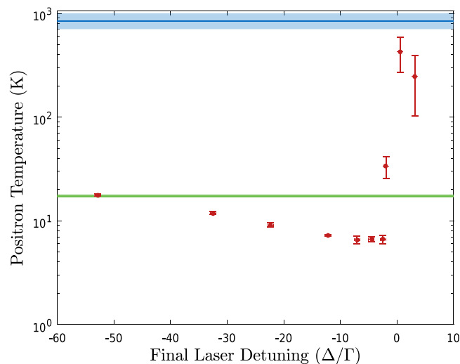
Fig. 2 Axial \text{e}^+ temperature in a mixed \text{Be}^+/\text{e}^+ plasma as a function of the final detuning ( \Delta ) of the \text{Be}^+ cooling laser. The mixed plasma consisted of 2.6 \times 10^6 \text{e}^+ , with an initial radius and density of 0.64 mm and 3 \times 10^8 \text{cm}^{-3} , respectively, and 3.8 \pm 0.1 \times 10^5 \text{Be}^+ ions. The laser frequency was swept from an initial detuning of -104\Gamma to the final laser detuning in -40 s. The error bars give the standard error of multiple measurements at each setting. The green line shows the \text{e}^+ temperature in the absence of any \text{Be}^+ ions ( 17.3 \pm 0.5 K), and the blue line shows the \text{e}^+ temperature when the laser is blocked and the \text{Be}^+ ions are not laser-cooled. The shading around these lines indicates the standard error.
