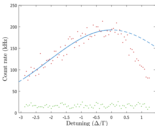
Fig. 10 Fluorescence signal from a pure \text{Be}^+ plasma as the frequency of the cooling laser is scanned across the laser cooling transition. The background-corrected signal (red points) has been fit with a Voigt function (blue solid line) on the left-hand side of the peak. It is clear that the function fits poorly if it is continued onto the right-hand side of the peak (blue dashed line) where the fluorescence signal drops off rapidly. This sharp decay in signal is attributed to the heating of the ions when the laser detuning is on the blue side of the resonance. The Voigt profile corresponds to an ion temperature of \sim 150 mK. The background signal on the detector when no ions are loaded, which comes mainly from the scatter of the laser beam within the apparatus, is shown for reference (green points).
