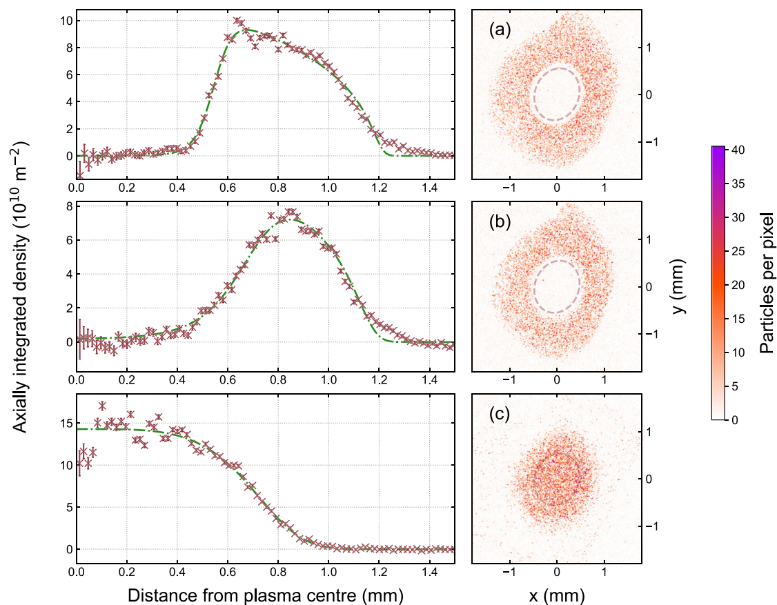
Fig. 4 \text{Be}^+ density profiles from originally mixed samples of \text{Be}^+ and \text{e}^+ with 2 \times 10^5 \text{Be}^+ and 1.2 \times 10^5 \text{e}^+ . The images (right) show \text{Be}^+ ejected to the MCP/Phosphor imaging assembly 5 \mu\text{s} after the ejection of \text{e}^+ in the opposite direction immediately following the laser-cooling of the \text{Be}^+ . a Laser detuning -20\Gamma , b Detuning -36\Gamma , and c Detuning -128\Gamma . The measured longitudinal temperatures were a 7.1 \pm 0.5 \text{ K} , b 10.1 \pm 0.2 \text{ K} , and c 370 \pm 100 \text{ K} , respectively. To the left of each image is a plot of the extracted axially integrated radial density profile, over-laid with the best fit distribution from calculations assuming thermal equilibrium at the temperatures stated. The fit results were a 6.2 \pm 0.6 \text{ K} , b 19 \pm 2 \text{ K} and c 253 \pm 54 \text{ K} . The corresponding \text{e}^+ densities were a , b 6.2 \pm 0.1 \times 10^7 \text{ cm}^{-3} and c 1.2 \pm 0.2 \times 10^8 \text{ cm}^{-3} . The calculations were done using the N2DEC code in ref. 34 , where thermal equilibrium of the two species is assumed. Note that due to the distortion in the imaging, the plasma image is elliptical; the extraction of the radial profile took this into account. Additionally, at higher radii ( >1.25 \text{ mm} ) the images are distorted by stray electric fields near the MCP as well as physical aperture effects.
