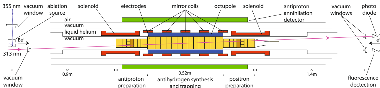
Fig. 1 ALPHA trap setup with \text{Be}^+ source and cooling laser. The main solenoid supplying a 1 T axial field throughout the center is not shown. The cylindrical electrodes (yellow/orange) can be individually charged to provide the axial electric fields for confinement. The central part is to scale. The short solenoids on either end can increase the axial field to 3 T in those regions. In typical operating conditions the field strength is homogenous to 1 part in 10^4 across a cylindrical region of \phi 6 mm \times 60 mm in the center 40 . The positron source and MCP/Phosphor assembly are to the right of the figure but not shown.
