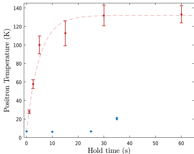
Fig. 5 Evolution of the e^+ temperature following the laser cooling frequency sweep. 1.4 \times 10^6 e^+ and 4.7 \pm 0.1 \times 10^5 Be^+ ions were used. Turning the cooling laser off (red points) results in the e^+ heating at a rate of \sim 25 K s^{-1} , before their temperature saturates at around 125 K. If, however, the cooling laser is kept on at a fixed detuning of -7\Gamma , the final detuning in the frequency sweep, the e^+ can be kept at 6.7 \pm 0.3 K for over 20 s (blue points). The vertical error bars correspond to the standard error on the mean temperature for each hold time.
