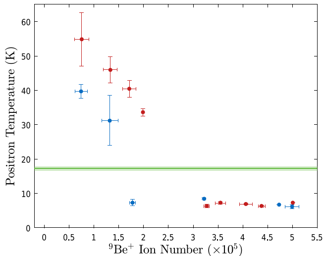
Fig. 3 Positron temperature as a function of the number of \text{Be}^+ ions used for sympathetic cooling. The ion number has been binned with the horizontal error bars representing the standard deviation of the mean ion number within each bin. The vertical error bars correspond to the standard error on the mean temperature within each bin. The ion number was varied by changing the number of ablation pulses used for loading, and also by splitting the ion plasma using axial potential manipulations. We used 1.4 \times 10^6 positrons (blue points) and 2.6 \times 10^6 positrons (red points) with initial densities of 1 \times 10^8 and 3 \times 10^8 \text{ cm}^{-3} , respectively. The cooling laser frequency was swept from an initial detuning of -129\Gamma to a final detuning of -7\Gamma in \sim 40 s for sympathetic cooling of the positrons. The positron temperature for 2.6 \times 10^6 positrons with no ions present (green line) is shown for comparison. The shading around this line indicates the standard error. Note that the positron-only temperature for 1.4 \times 10^6 positrons is consistent with this temperature.
