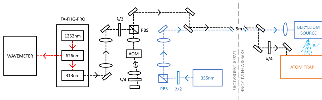
Fig. 9 Laser-setup for ablation (blue) and laser-cooling (black). The TA-FHG PRO from Toptica generates 313 nm by two doubling stages of a 1252 nm amplified diode laser. The second harmonic light at 626 nm is sent to a wavemeter for frequency control (see below). The double-pass AOM setup is used to sweep the laser for fluorescence-based detection (the detection geometry was indicated in Fig. 1). The polarization beam splitters (PBS) for both lasers serve, through changes of polarization to control the power delivered to the experiment. Both lasers are passed through a periscope setup from the laser room to the experiment. The quarter-wave plate on the 313 nm path before it enters the Atom Trap serves to tune the polarization.
