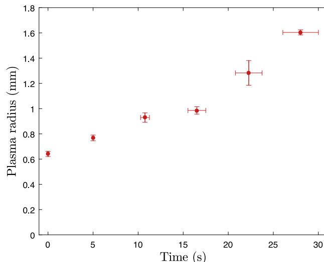
Fig. 7 Evolution of the radius of the positron plasma as a function of time during the laser cooling frequency sweep. The plasma was a mixture of 2.6 \times 10^6 e^+ and \sim 4-5 \times 10^5 Be^+ ions. Time zero is when the frequency sweep begins. The total sweep time we use to sympathetically cool the positrons to their lowest temperatures is 40 s. It is not possible to measure plasma radii greater than around 1.6 mm with our current MCP imaging diagnostic. The error corresponds to the standard error on the mean radius measured (vertical bars) and the laser-cooling time (horizontal).
