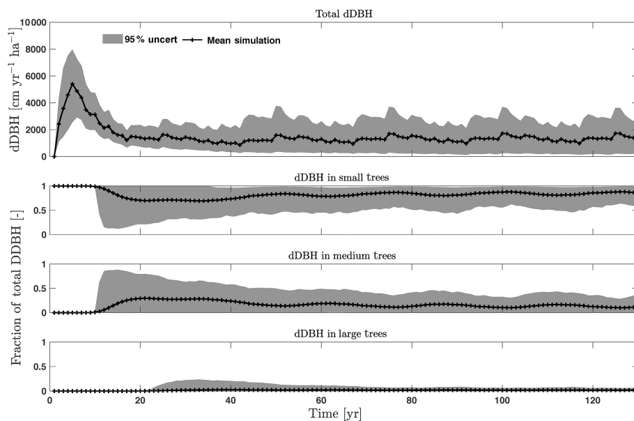
Figure D2. Simulated total change in diameter at breast height (dDBH) from CLM4.5(FATES) for all trees and its fractional distribution for small (diameter < 10\text{ cm} ), medium ( 10\text{ cm} < \text{diameter} < 50\text{ cm} ), and large trees (diameter > 50\text{ cm} ). Shown is the mean simulation (black line) with 95 % spread of the simulation ensemble.
