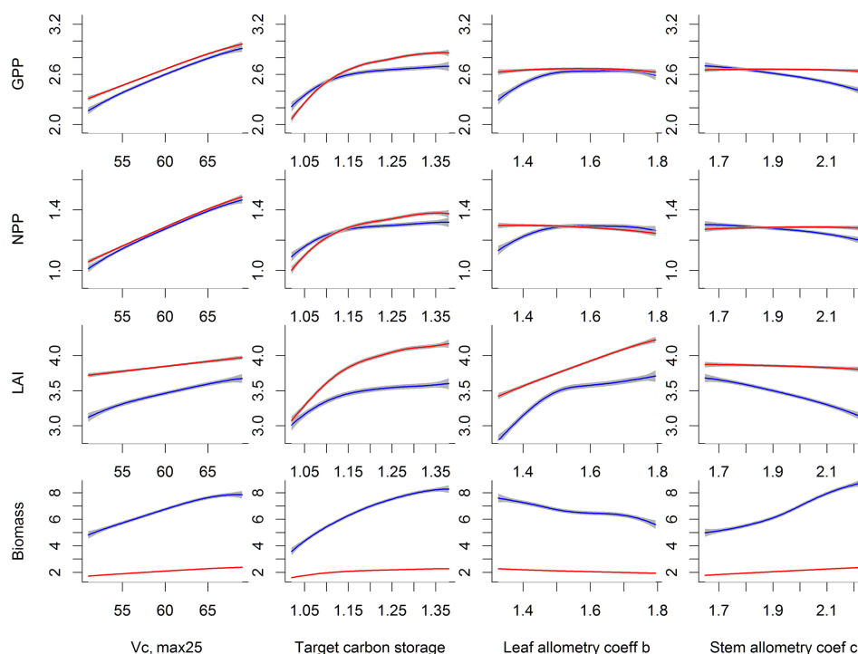
Figure 8. Relations between outputs of CLM4.5(FATES), including GPP, NPP, LAI, and biomass (units shown in Fig. 6), and the most sensitive parameters, i.e., V_{c,\max25} (units are \mu\text{mol CO}_2 \text{ m}^{-2} \text{ s}^{-1} ), target storage carbon (unit is the ratio of leaf biomass), leaf and stem allocation (unitless parameters) for simulation year 10 (red) and 130 (blue). Shown are the mean relations with the 95 % confidence intervals in grey envelopes. These figures show how an output will generally increase or decrease when a given parameter is changed.
