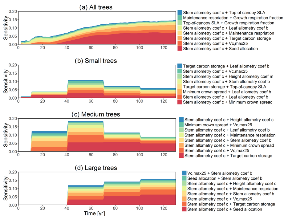
Figure D7. Second-order sensitivity index of the model parameters for the basal area (BA) outputs from CLM4.5(FATES) for (a) all trees, (b) small trees, (c) medium trees, and (d) large trees. Shown are the top eight most important parameter interactions in order of importance based on the mean parametric sensitivity across years (red is the most important and blue is the least important)
