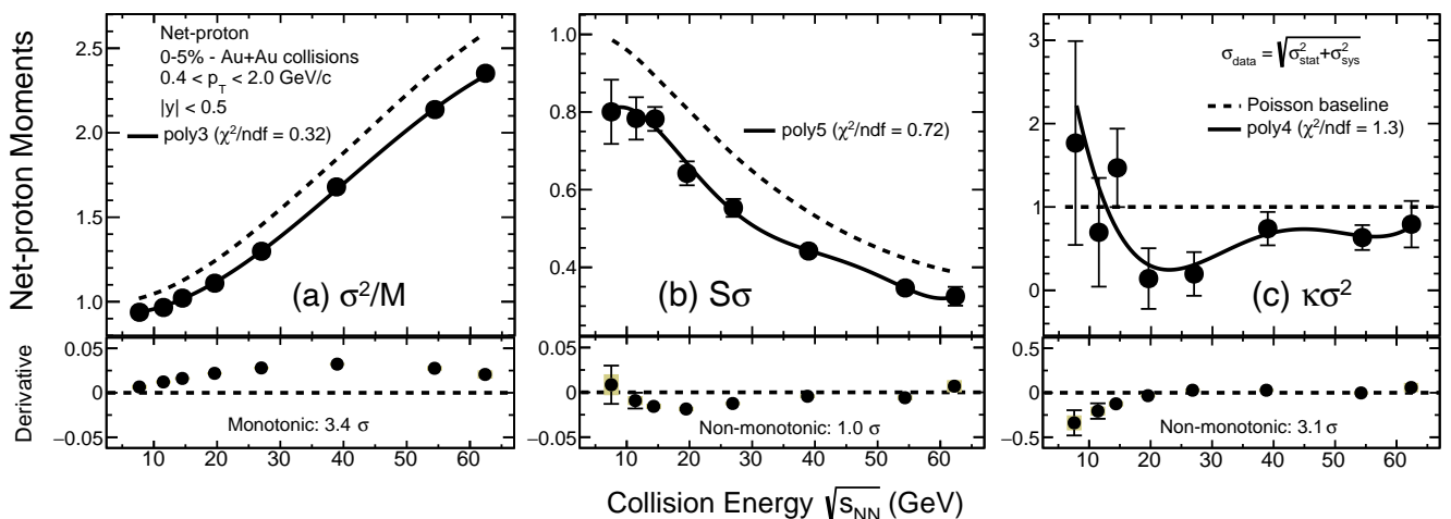
FIG. 23. (Color online) Upper panel: (a) \sigma^2/M , (b) S\sigma and (c) \kappa\sigma^2 of net-proton distributions for 0-5% central Au+Au collisions from \sqrt{s_{\text{NN}}} = 7.7 - 62.4 GeV. The error bars on the data points are statistical and systematic uncertainties added in quadrature. The black solid lines are polynomial fit functions which well describe the cumulant ratios. The legends also specify the values of chi-squared per degree of freedom for the respective fits. The black dashed lines are the Poisson baselines. Lower panel: Derivative of the fitted polynomial as a function of collision energy. The bar and the gold band on the derivatives represent the statistical and systematic uncertainties, respectively.
