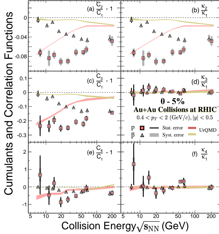
FIG. 25. (Color online) Collision energy dependence of the scaled (anti)proton cumulants and correlation functions in 0-5% central Au+Au collisions at \sqrt{s_{\text{NN}}} = 7.7, 11.5, 14.5, 19.6, 27, 39, 54.4, 62.4, and 200 GeV. The error bars and bands represent the statistical and systematic uncertainties, respectively. The results from UrQMD model calculation are also shown for comparison.
