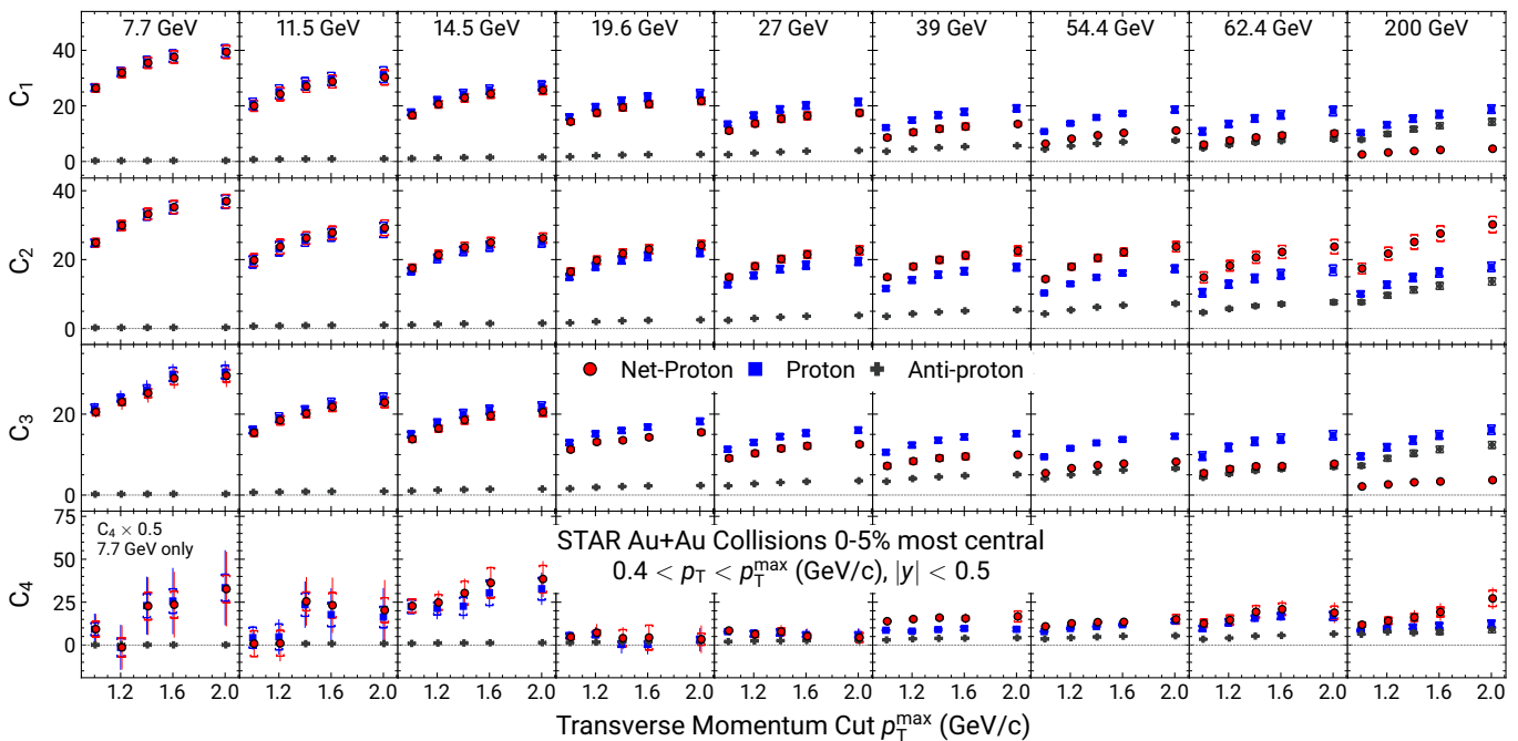
FIG. 18. (Color online) p_T -acceptance dependence of cumulants of proton, antiproton and net-proton multiplicity distributions for 0-5% central Au+Au collisions at \sqrt{s_{\text{NN}}} = 7.7, 11.5, 14.5, 19.6, 27, 39, 54.4, 62.4 and 200 GeV. The bars and caps represent statistical and systematic uncertainties, respectively. For clarity, the X -axis values for net-protons are shifted and the values of proton, antiproton and net-proton C_4 at \sqrt{s_{\text{NN}}} = 7.7 GeV are scaled down by a factor of 2.
