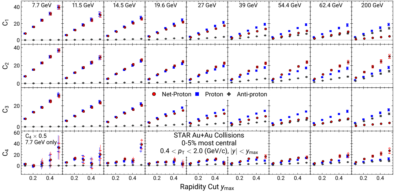
FIG. 15. (Color online) Rapidity acceptance dependence of cumulants of proton, antiproton and net-proton multiplicity distributions in 0-5% central Au+Au collisions at \sqrt{s_{\text{NN}}} = 7.7, 11.5, 14.5, 19.6, 27, 39, 54.4, 62.4 and 200 GeV. The bars and caps represent statistical and systematic uncertainties, respectively. For clarity, the X-axis values for protons are shifted and the values of proton, antiproton and net-proton C_4 at \sqrt{s_{\text{NN}}} = 7.7 GeV are scaled down by a factor of 2.
